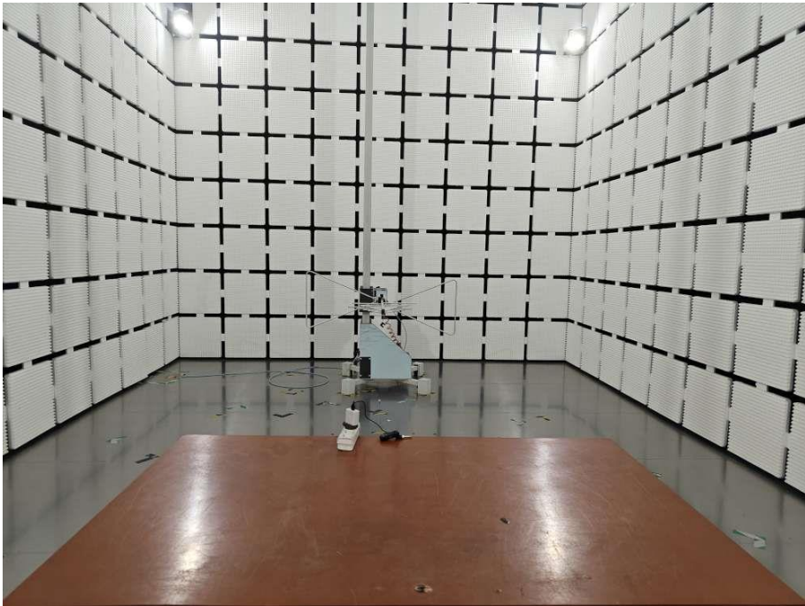
Radiated Emission Test View Below 1GHz 2
