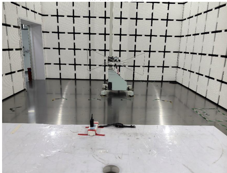
Radiated Emission
