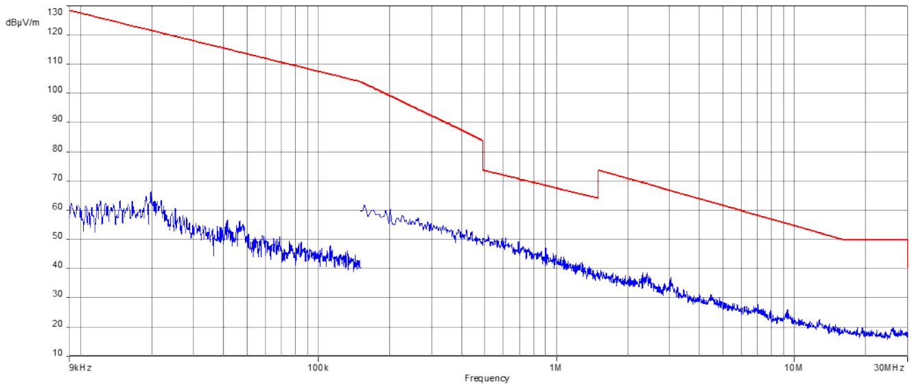
Plot 1: 1030 MHz, cabinet radiation (valid for all modes), 9 kHz – 30 MHz
