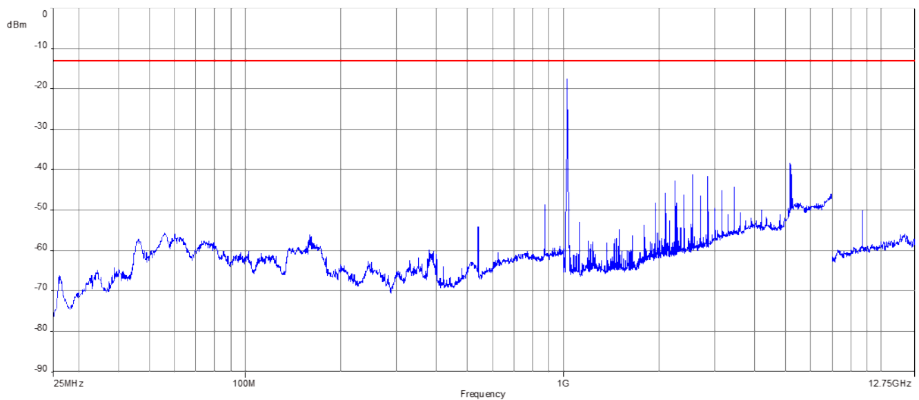
Plot 2: 1030 MHz, cabinet radiation (valid for all modes), 25 MHz – 12.75 GHz
