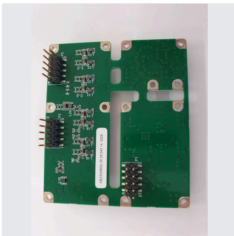
Photo 8 Down Converter Board bottom
