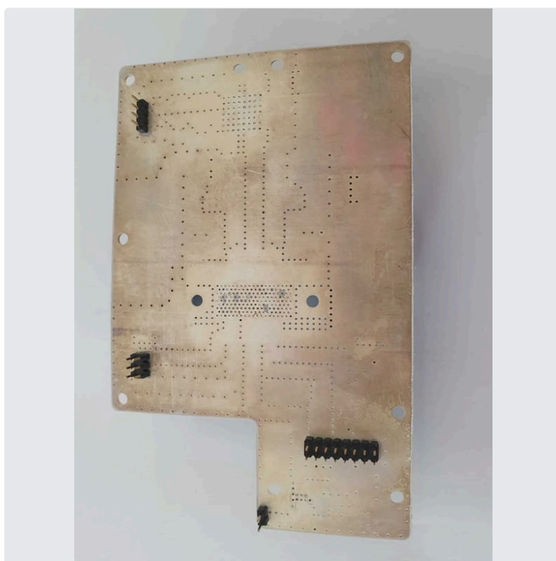
Photo 18 RF Amp Board bottom
