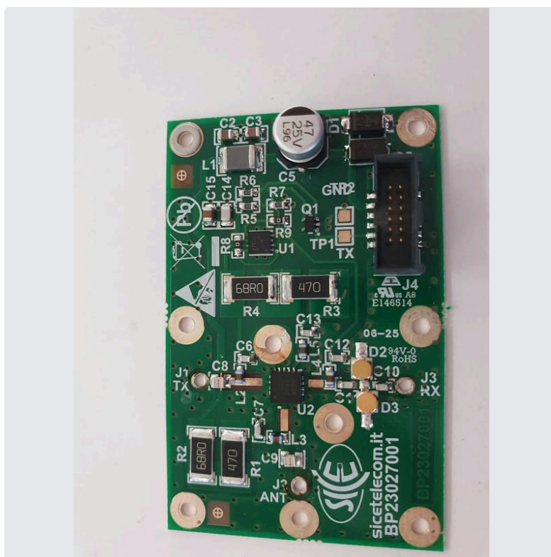
Photo 19 RF Switch Board top
