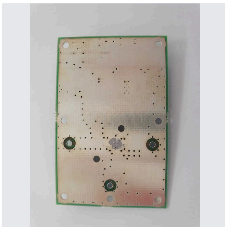
Photo 20 RF Switch Board bottom
