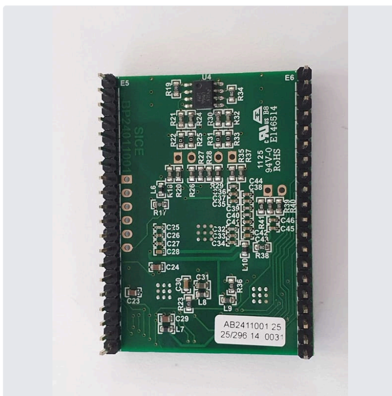
Photo 22 Shaper Board bottom
