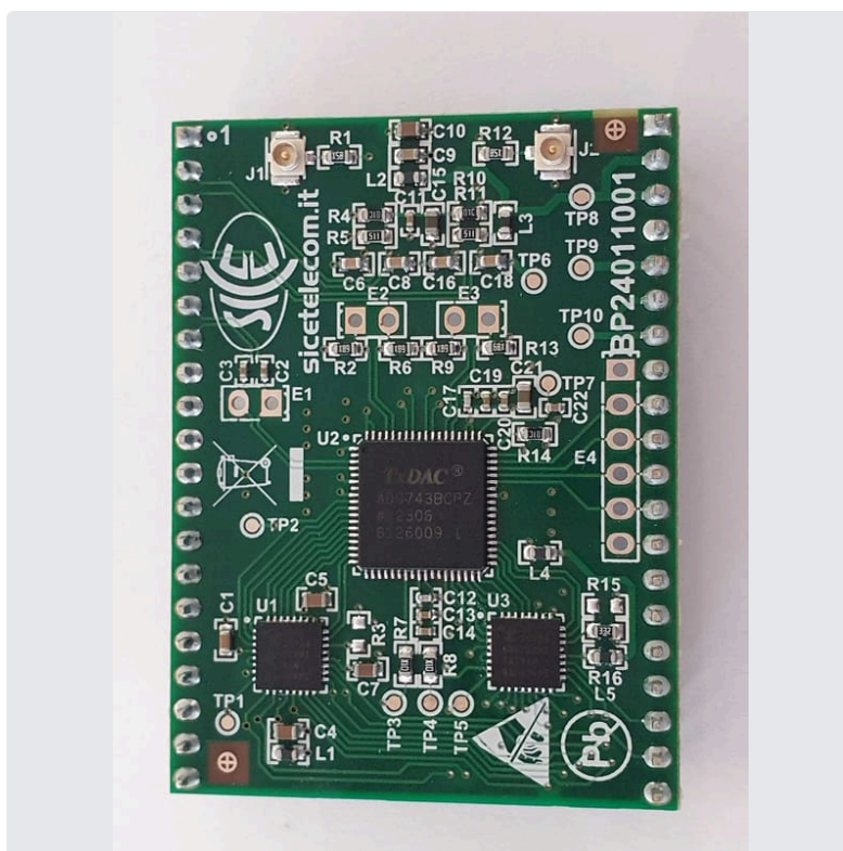
Photo 21 Shaper Board top
