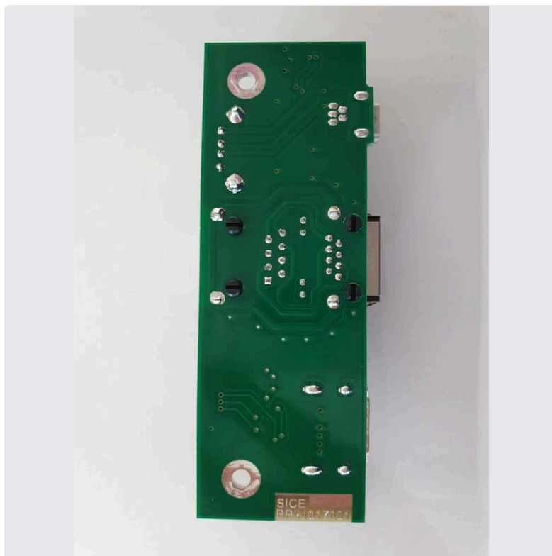
Photo 1 Connectors Board bottom
