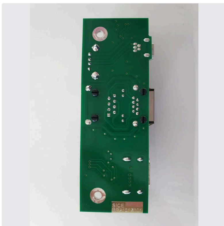
Photo 2 Connectors Board bottom
