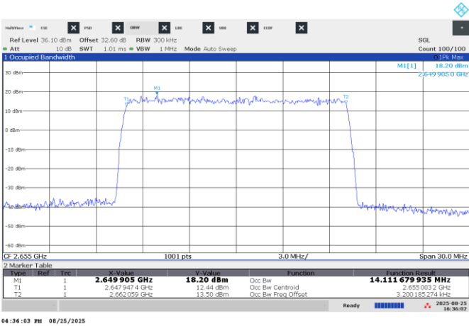
Figure 8.11-5: Sample plot for NR 15 MHz Channel
