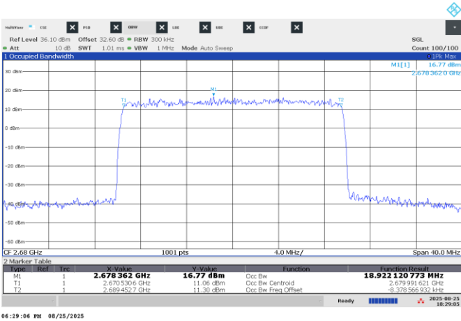
Figure 8.11-6: Sample plot for NR 20 MHz Channel
