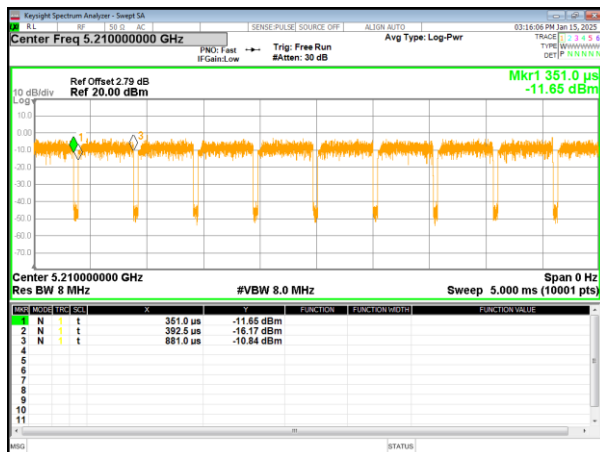
(802.11ax80) plot
