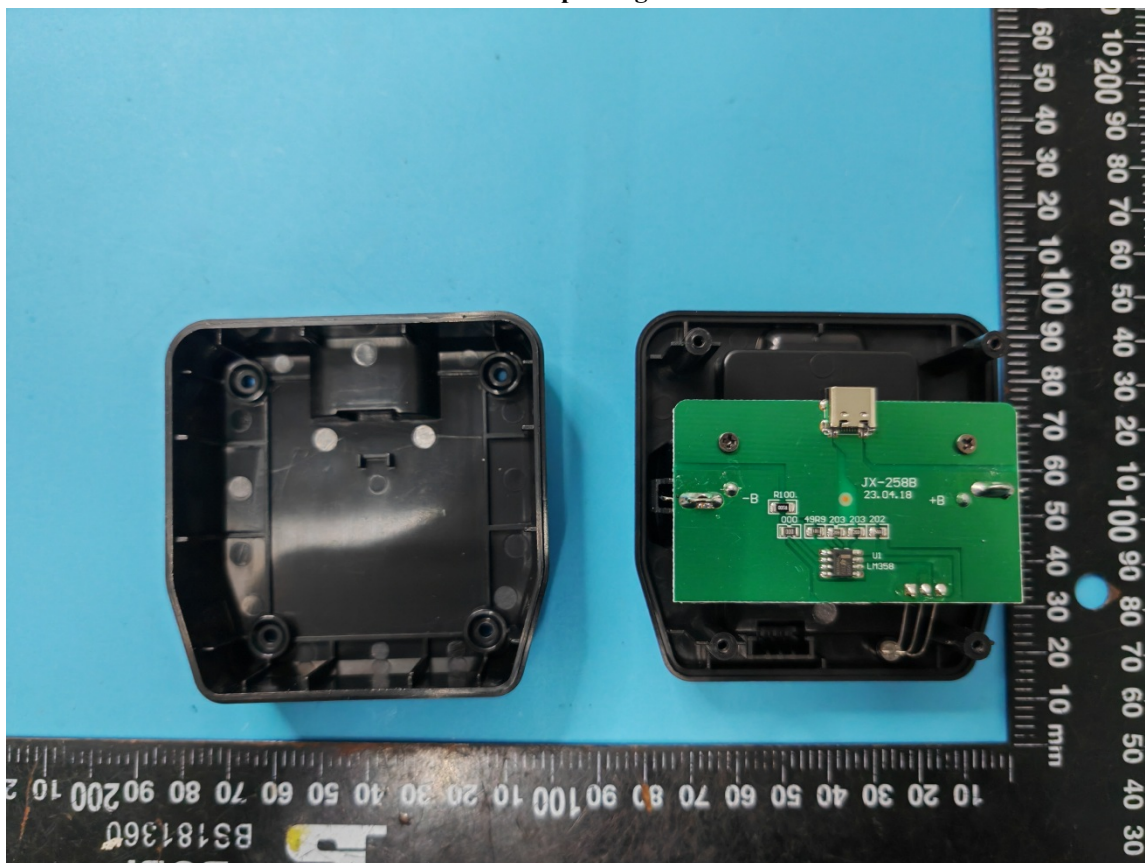
desktop charger
