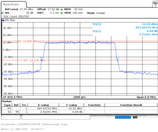
26dB Bandwidth
