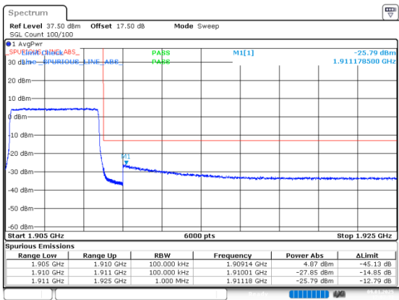
5MHz_High_16QAM_25@0
