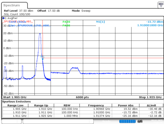
5MHz_High_QPSK_1@24
