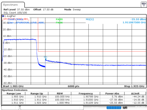
5MHz_High_QPSK_25@0
