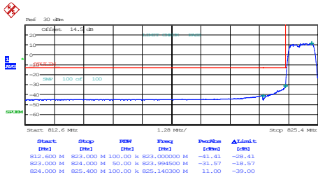
1.4MHz_Low_QPSK_6@0
