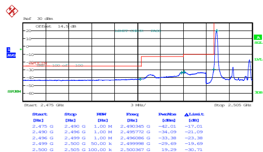
5MHz_Low_16QAM_1@0
