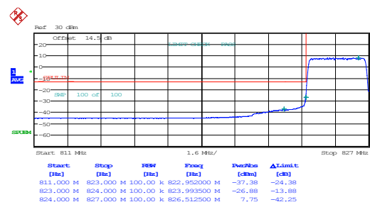
3MHz_Low_QPSK_15@0
