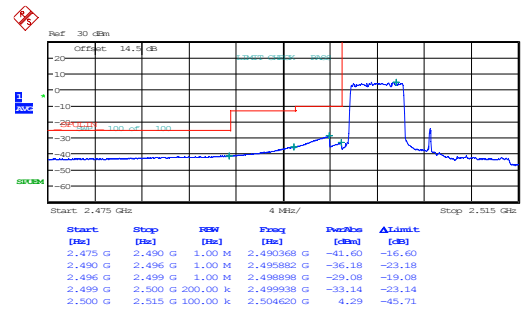
15MHz_Low_16QAM_25@0
