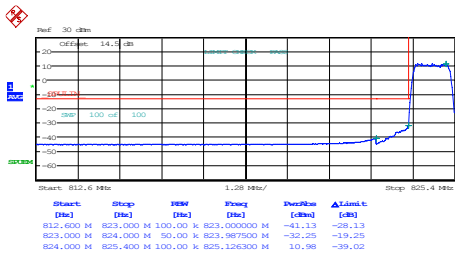
1.4MHz_Low_16QAM_6@0
