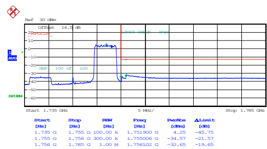
20MHz_High_16QAM_25@75
