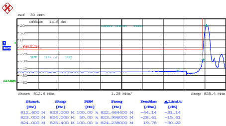
1.4MHz_Low_16QAM_1@0
