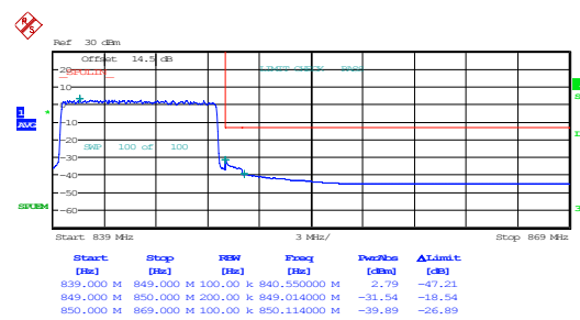
10MHz_High_QPSK_50@0
