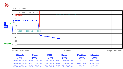
5MHz_High_16QAM_25@0
