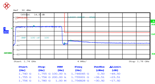
15MHz_High_QPSK_75@0
