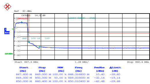
1.4MHz_High_16QAM_6@0
