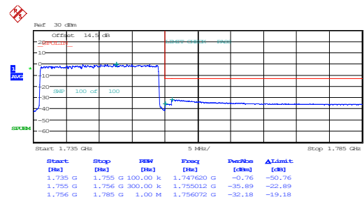
20MHz_High_QPSK_100@0
