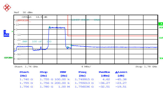
15MHz_High_16QAM_25@50
