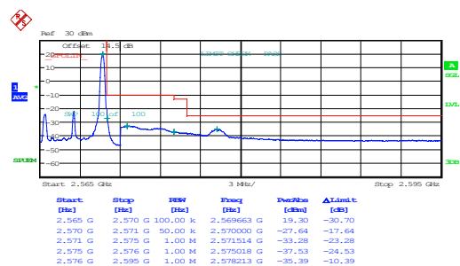
5MHz_High_QPSK_1@24
