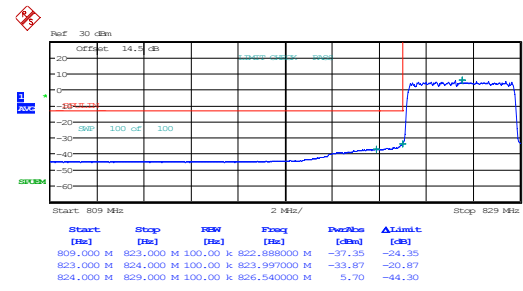
5MHz_Low_16QAM_25@0
