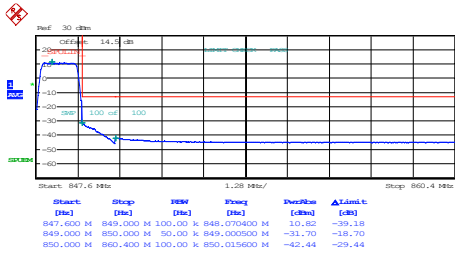
1.4MHz_High_QPSK_6@0
