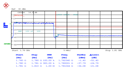
20MHz_High_QPSK_100@0
