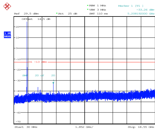
20MHz_High_QPSK_1@0(30MHz~18.55GHz)
