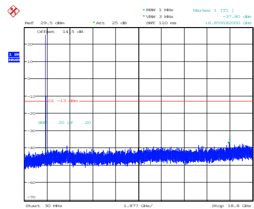
10MHz_High_QPSK_1@0(30MHz~18.8GHz)
