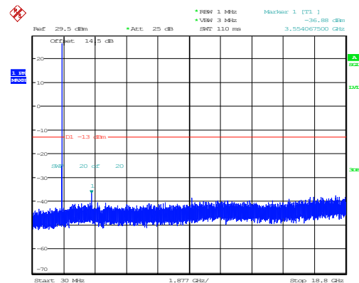
3MHz_High_QPSK_1@0(30MHz~18.8GHz)
