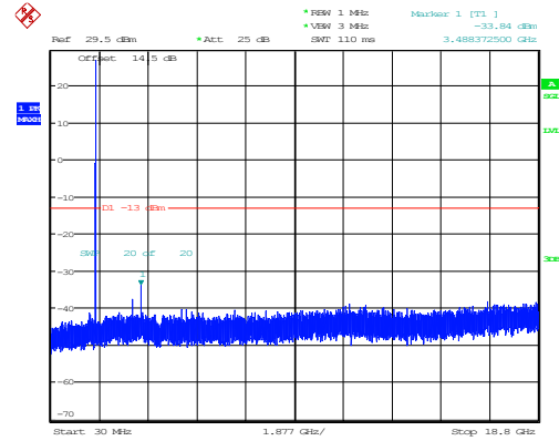
1.4MHz_Middle_QPSK_1@0(30MHz~18.8GHz)
