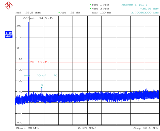
10MHz_Low_QPSK_1@0(30MHz~20.1GHz)
