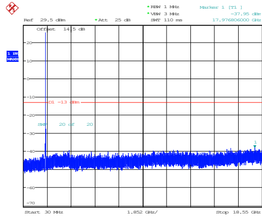
15MHz_Middle_QPSK_1@0(30MHz~18.55GHz)
