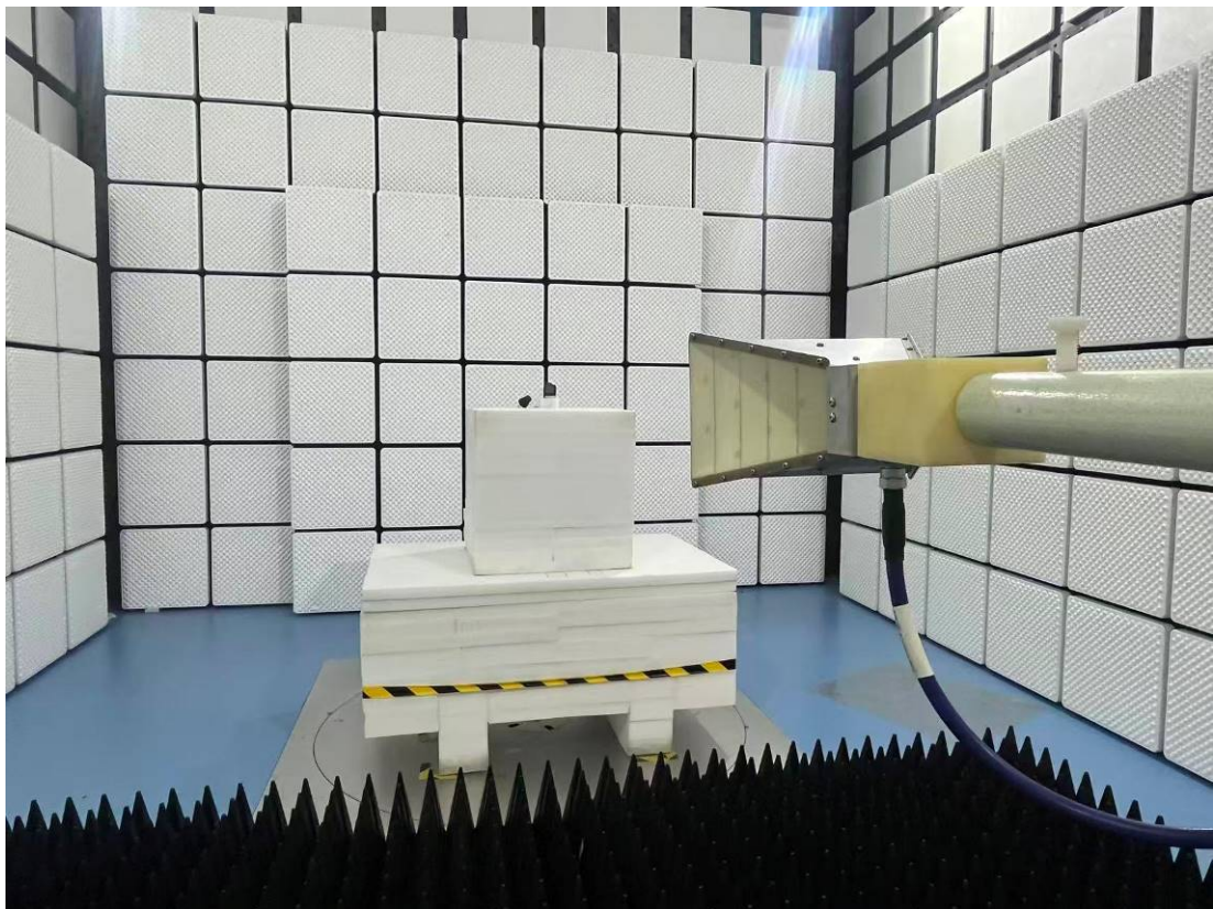
RE- Rear View (Above 1GHz)
