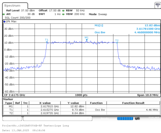
Occupied Bandwidth
