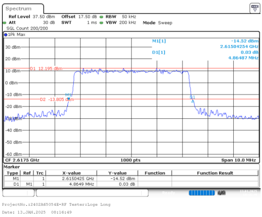
26dB Bandwidth
