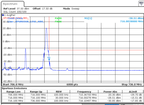
10MHz_High_QPSK_1@49
