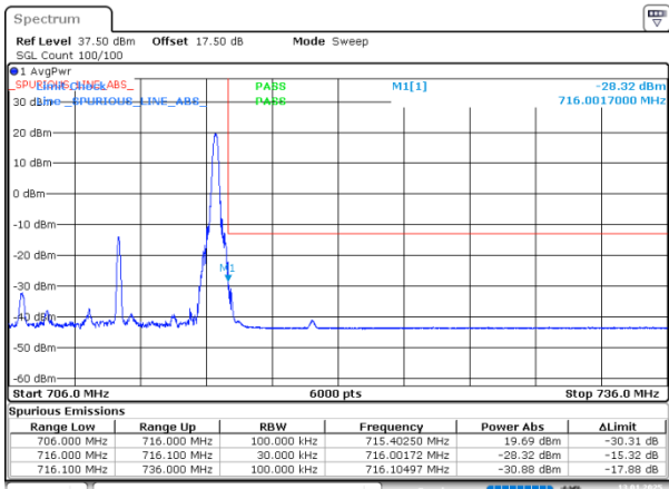
10MHz_High_16QAM_1@49
