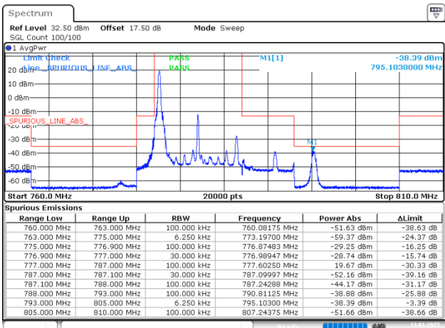
10MHz_Middle_QPSK_1@0
