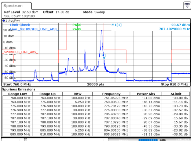
10MHz_Middle_QPSK_1@49
