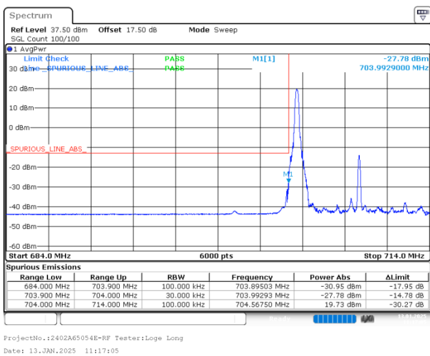
10MHz_Low_16QAM_1@0
