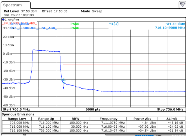
10MHz_High_16QAM_25@25
