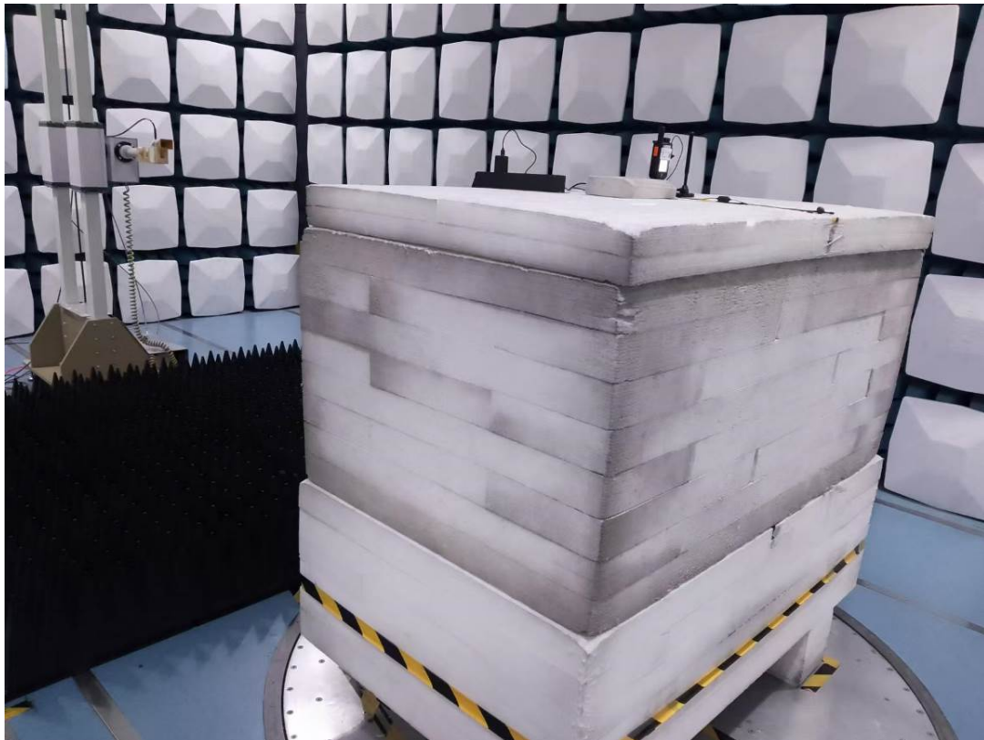
Radiated Emission 26.5-27GHz View
