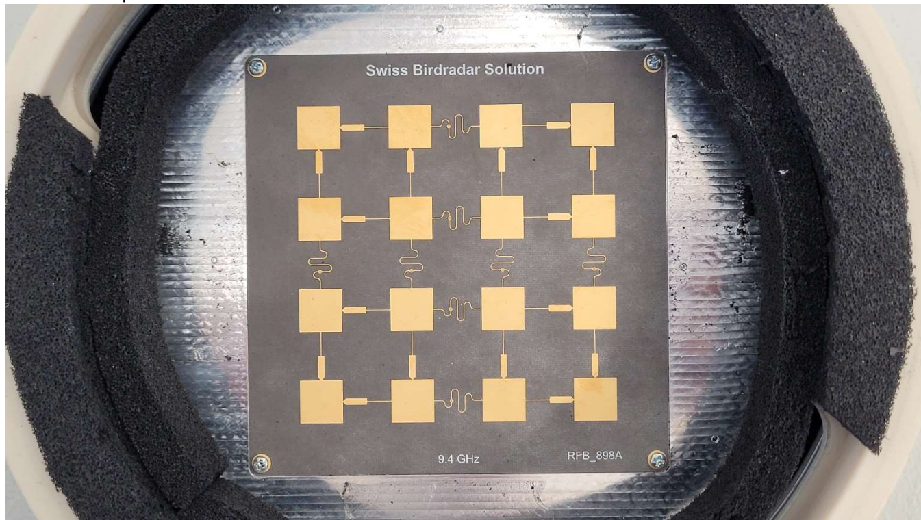
Photo No. 17: patch antenna
