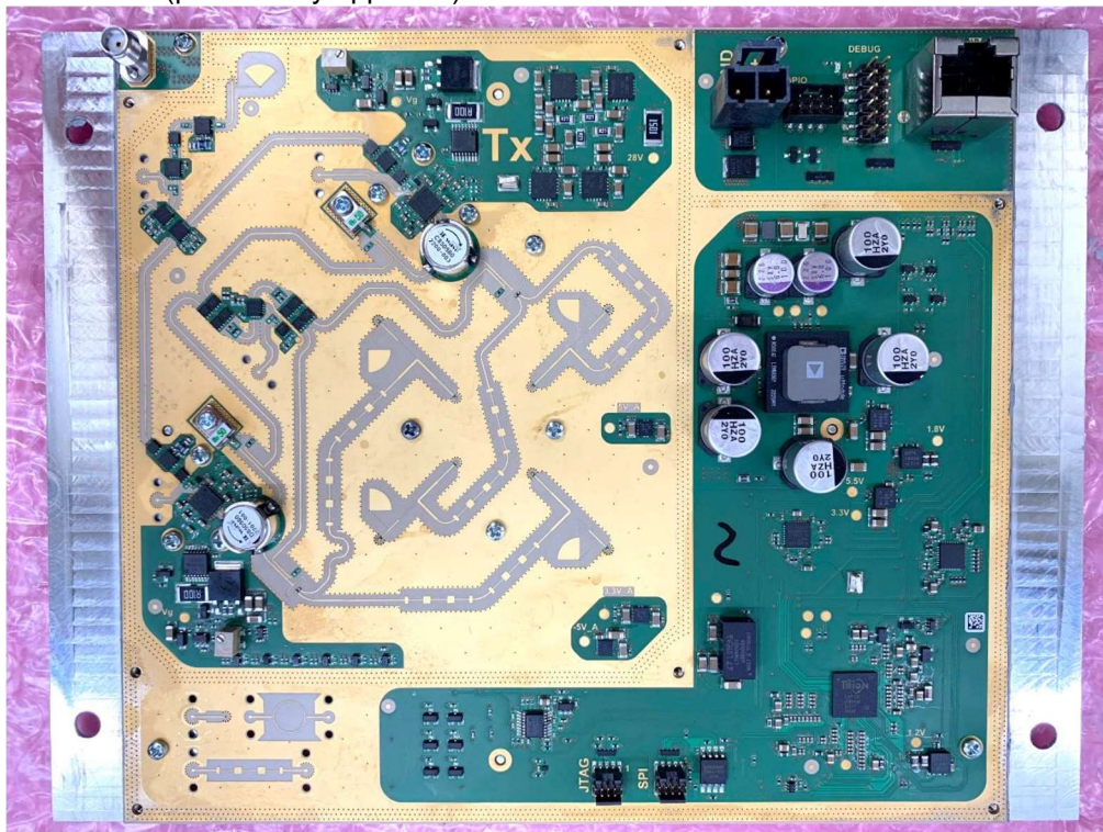
Photo No. 19: Transmitter (provided by applicant)
