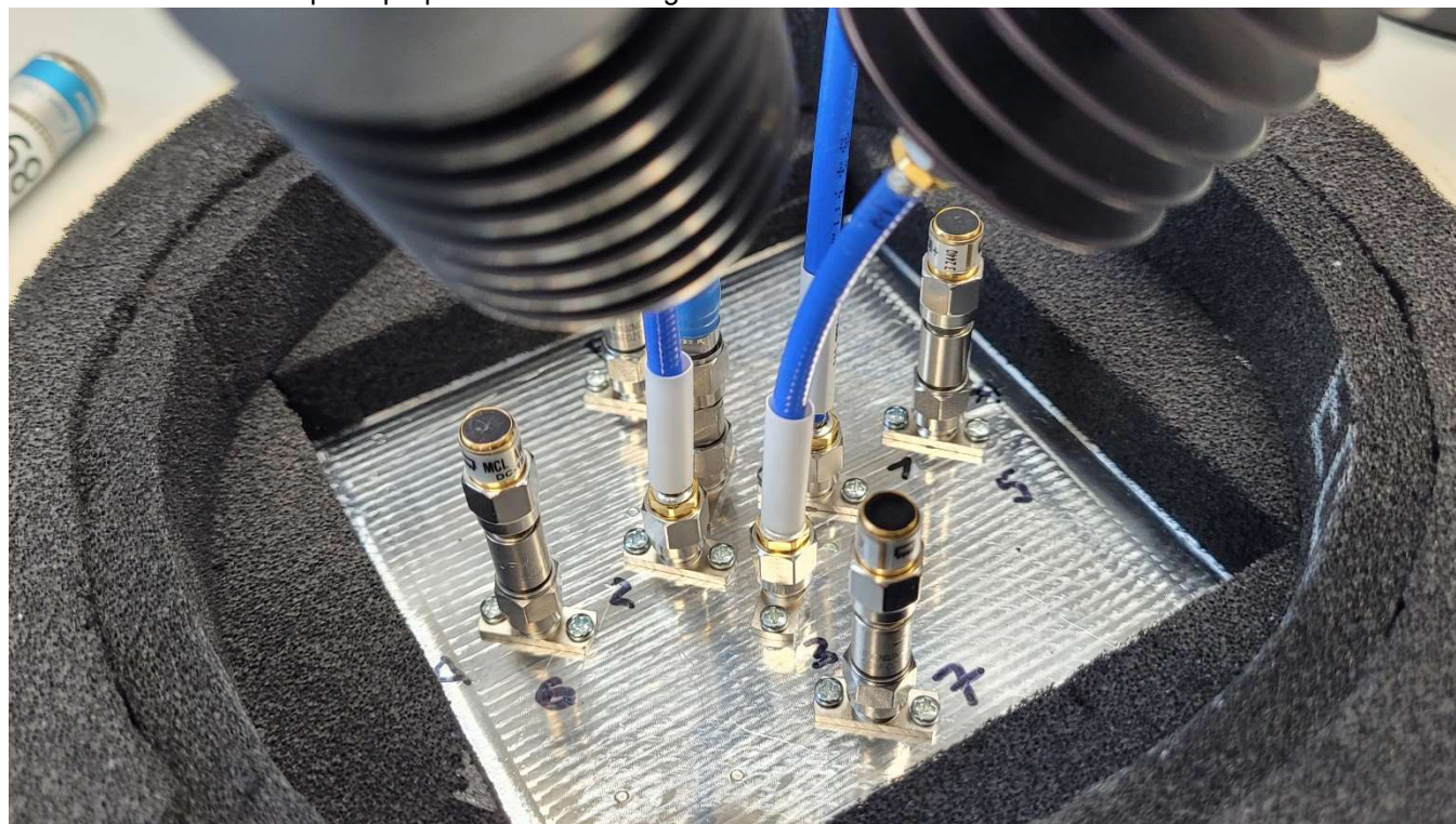
Photo No. 18: coax adapters prepared for RF testing
