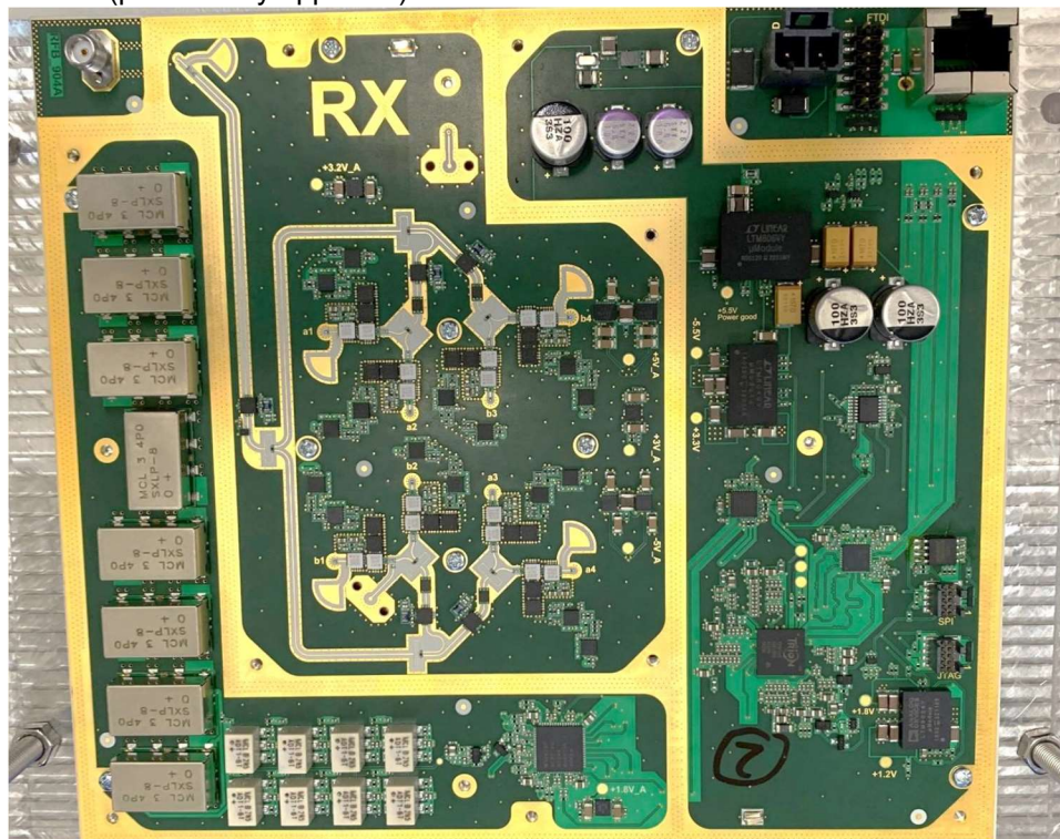
Photo No. 20: Receiver (provided by applicant)
