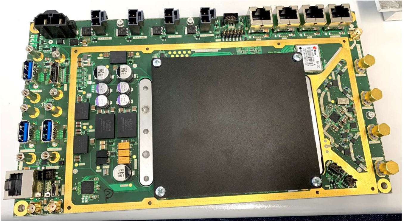
Photo No. 21: Signal Processing (provided by applicant)
