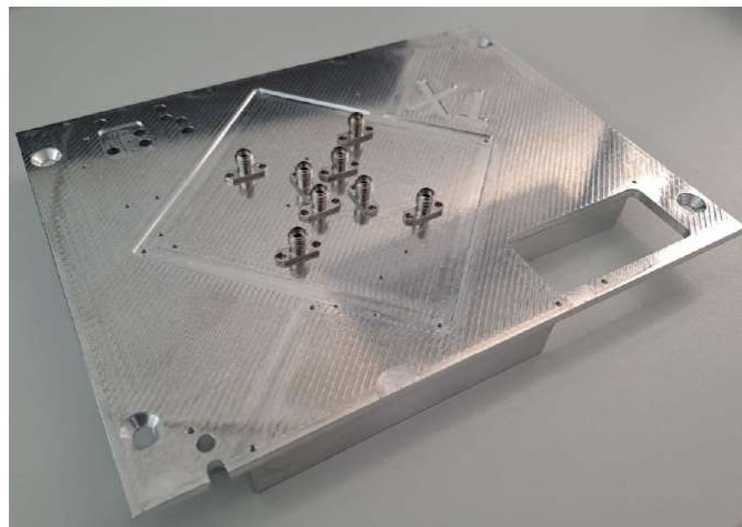
Figure 7: Transmitter with SMA connectors
