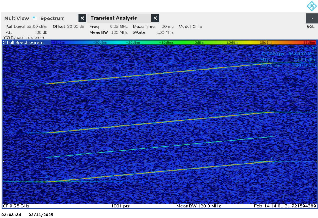
Plot no. 119: Timing CH3
