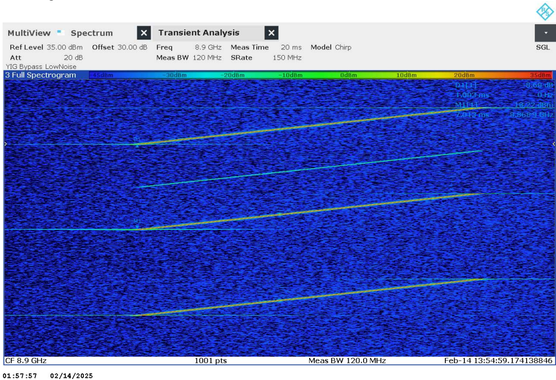
Plot no. 117: Timing CH2
