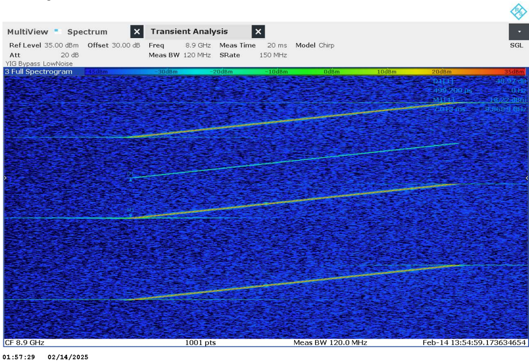
Plot no. 116: Timing CH2
