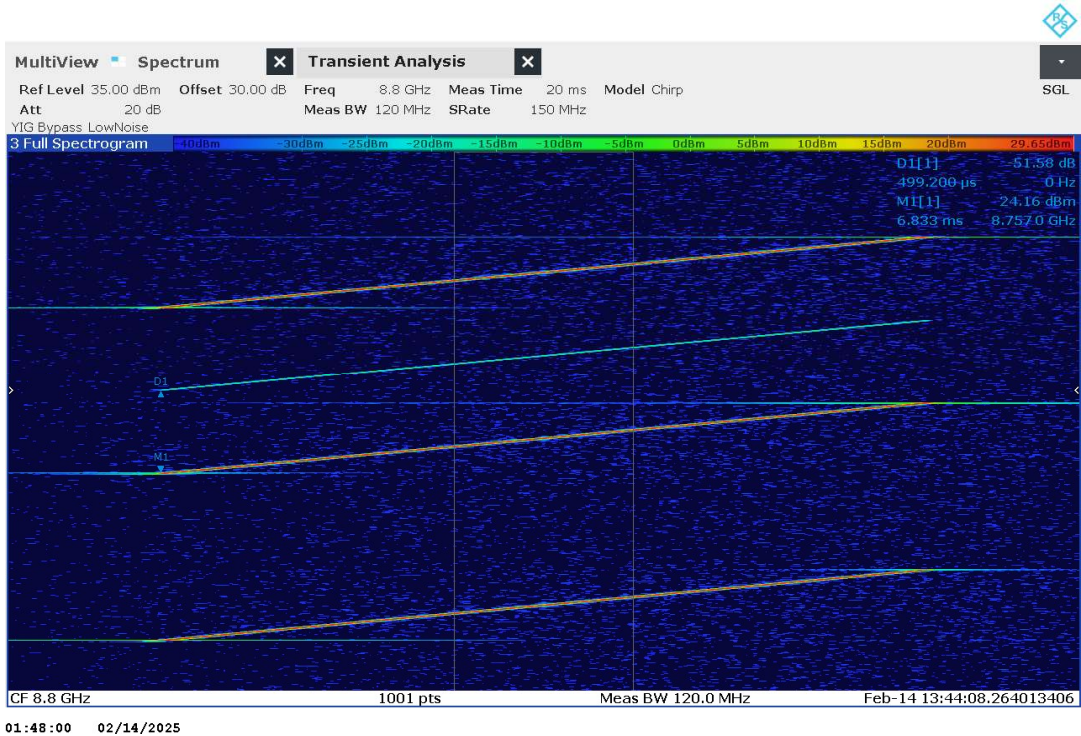
Plot no. 112: Timing CH1
