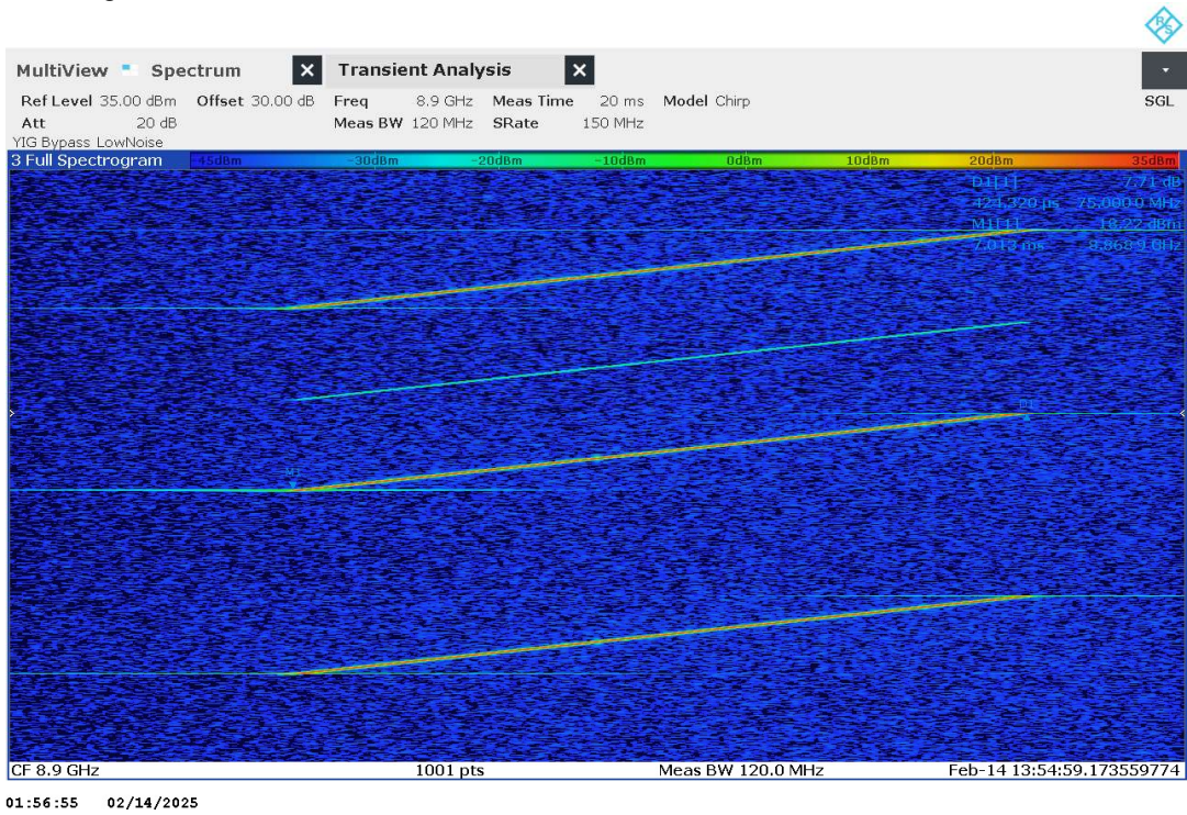
Plot no. 115: Timing CH2
