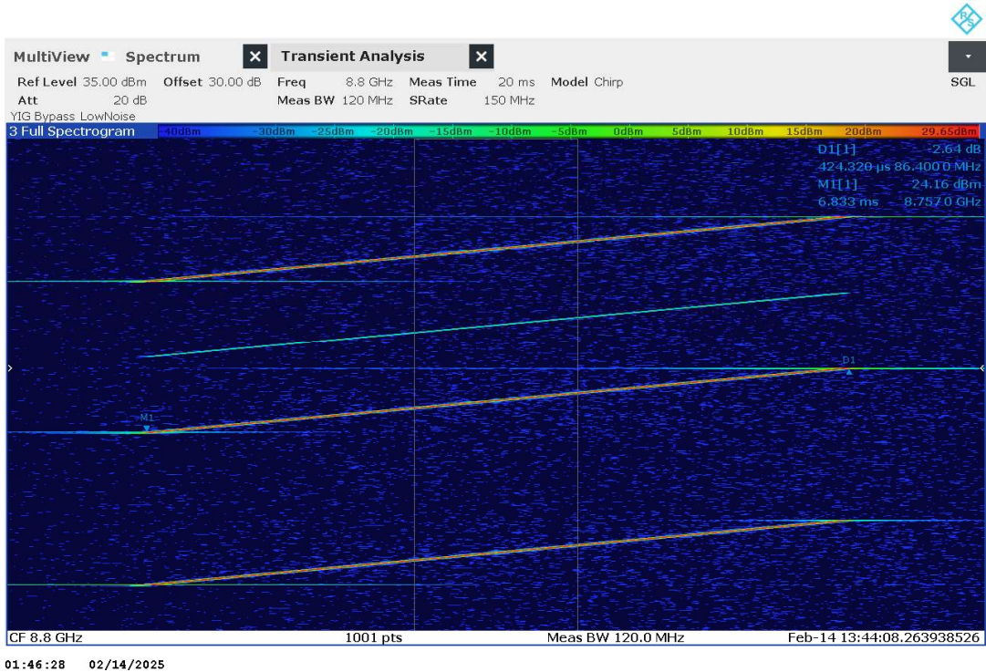
Plot no. 111: Timing CH1
