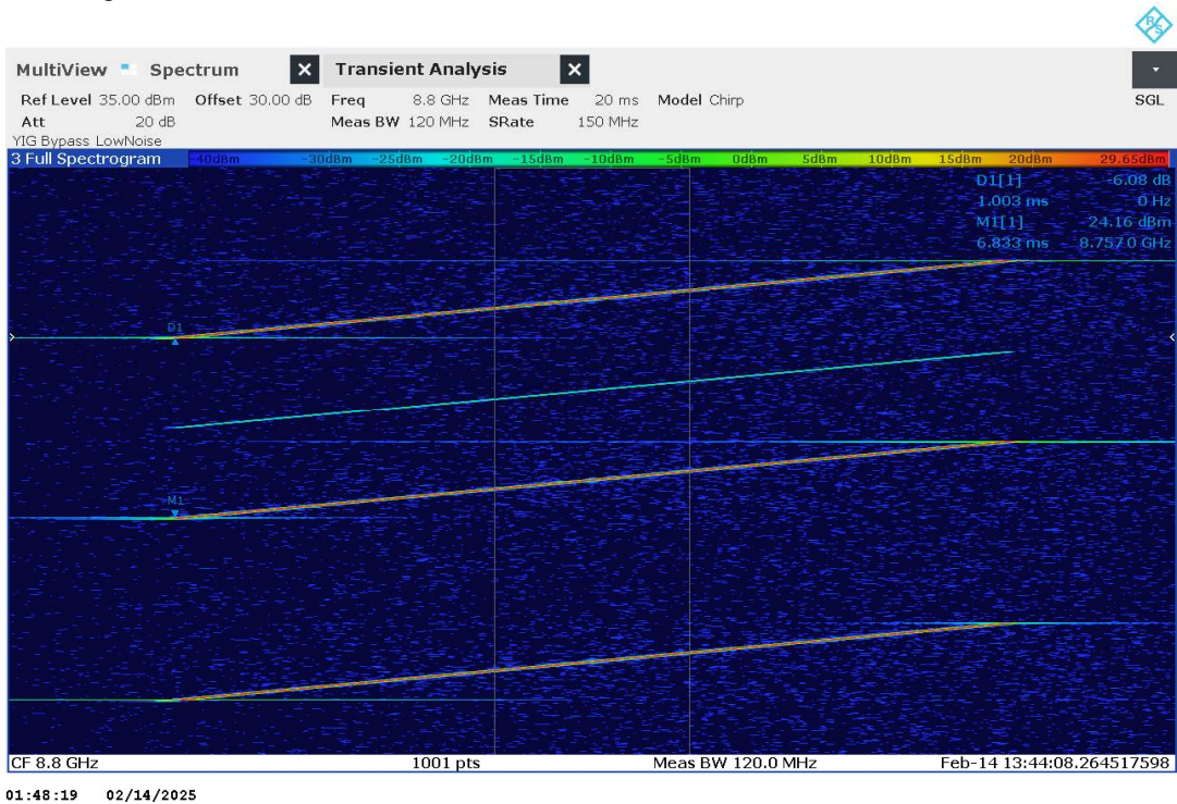
Plot no. 113: Timing CH1
