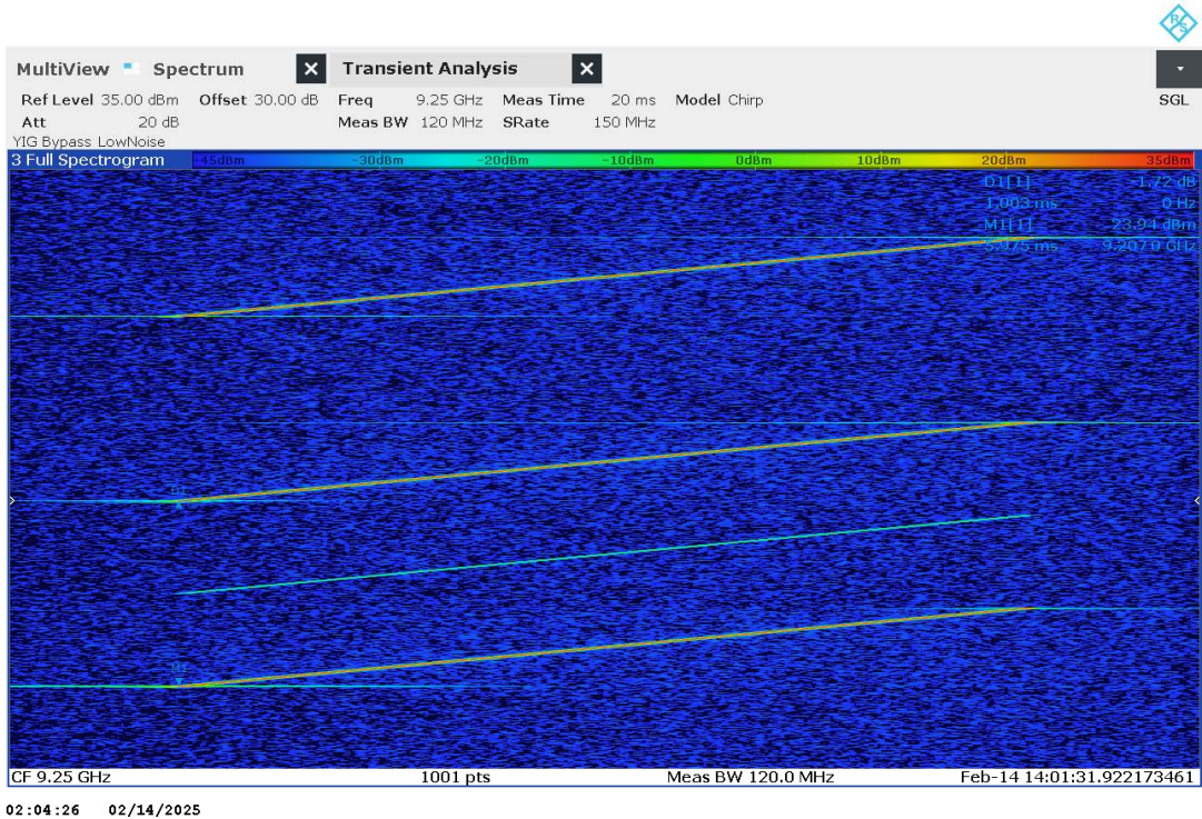
Plot no. 121: Timing CH3
