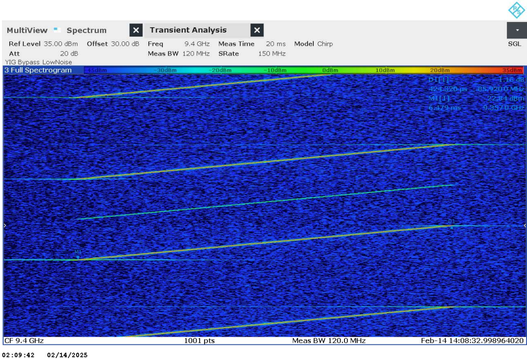
Plot no. 123: Timing CH4, 83 MHz
