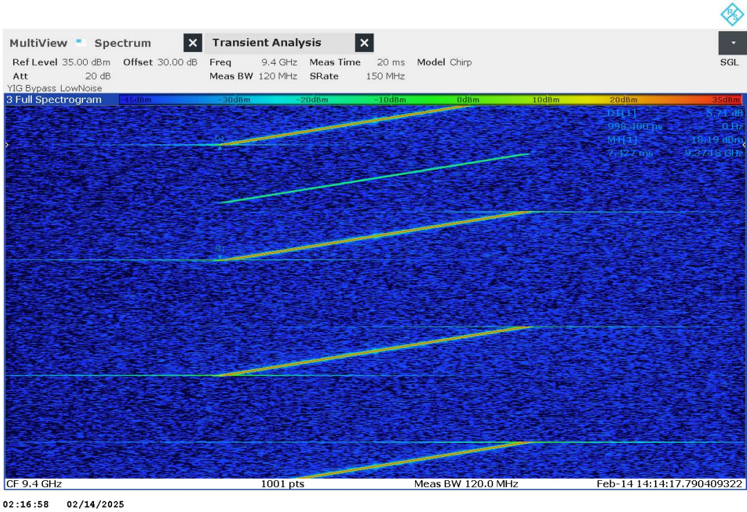
Plot no. 129: Timing CH4, 48 MHz
