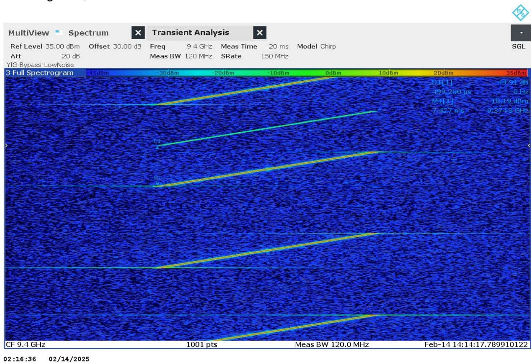
Plot no. 128: Timing CH4, 48 MHz
