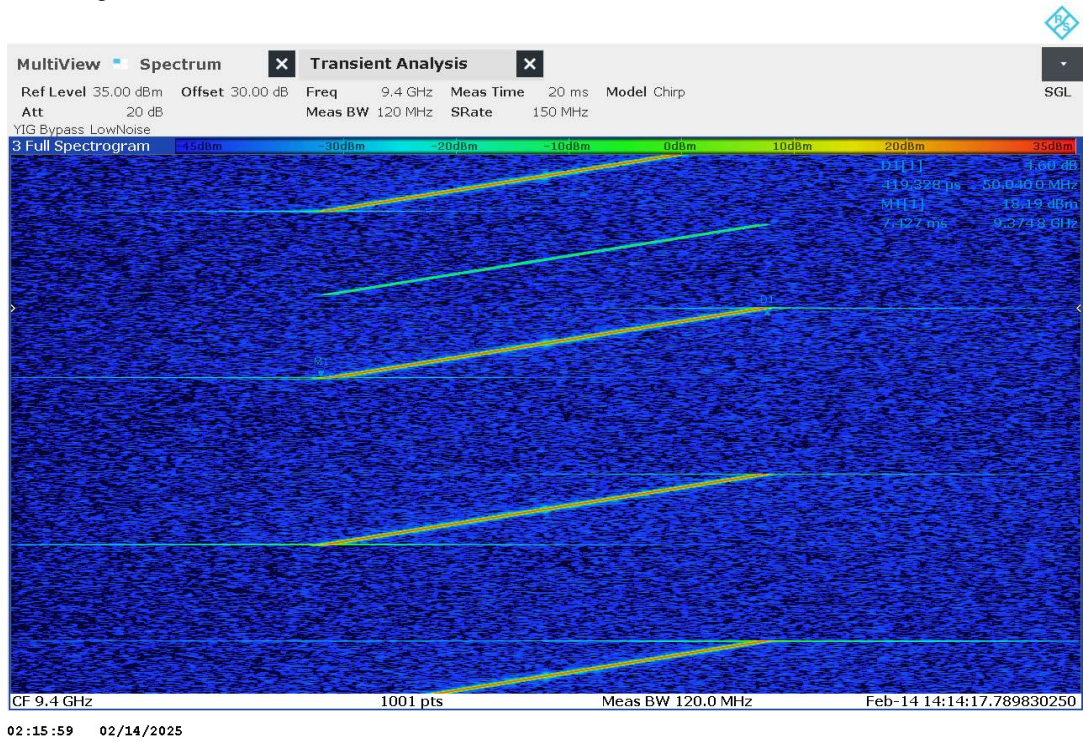
Plot no. 127: Timing CH4, 48 MHz
