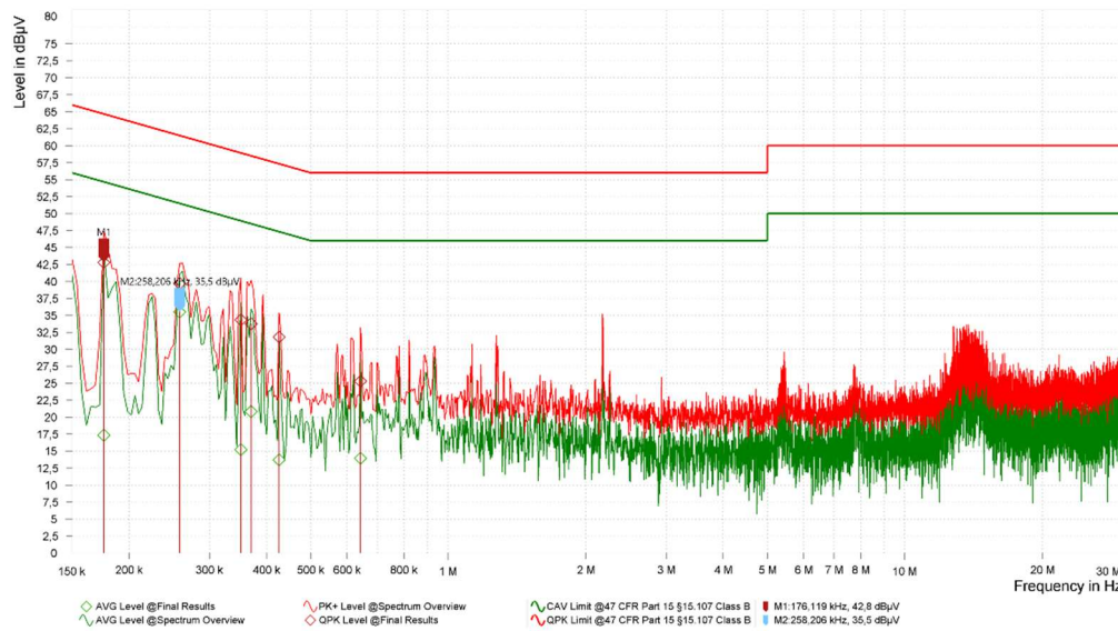
Plot no. 29: conducted emissions, neutral N, CH2
