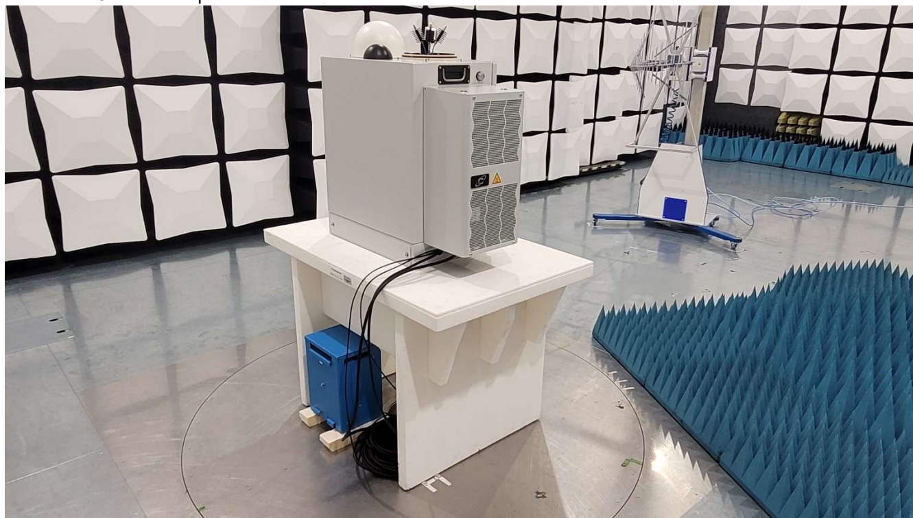
Photo No. 25: radiated spurious
