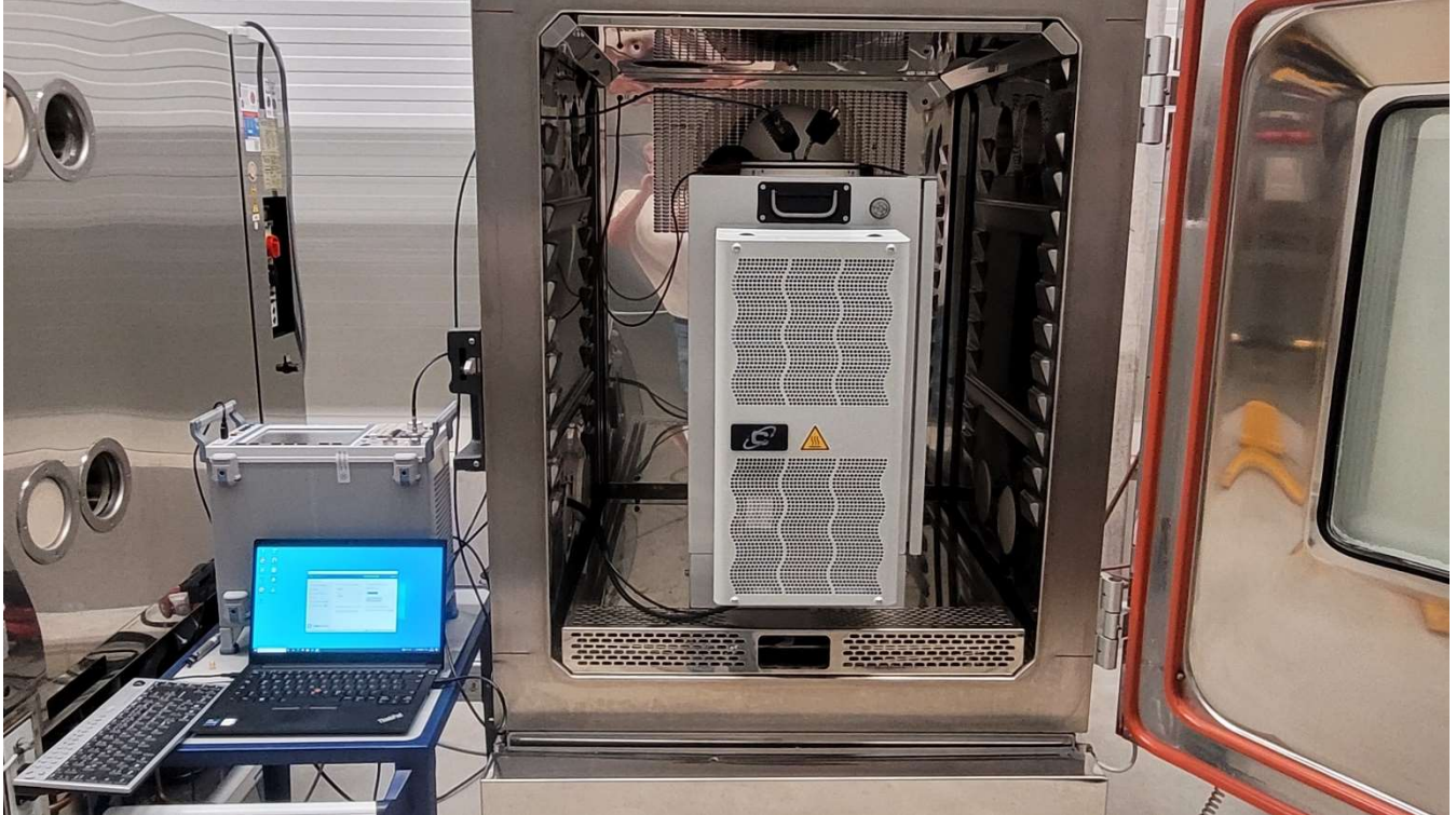
Photo No. 28: tests under extreme temperature
