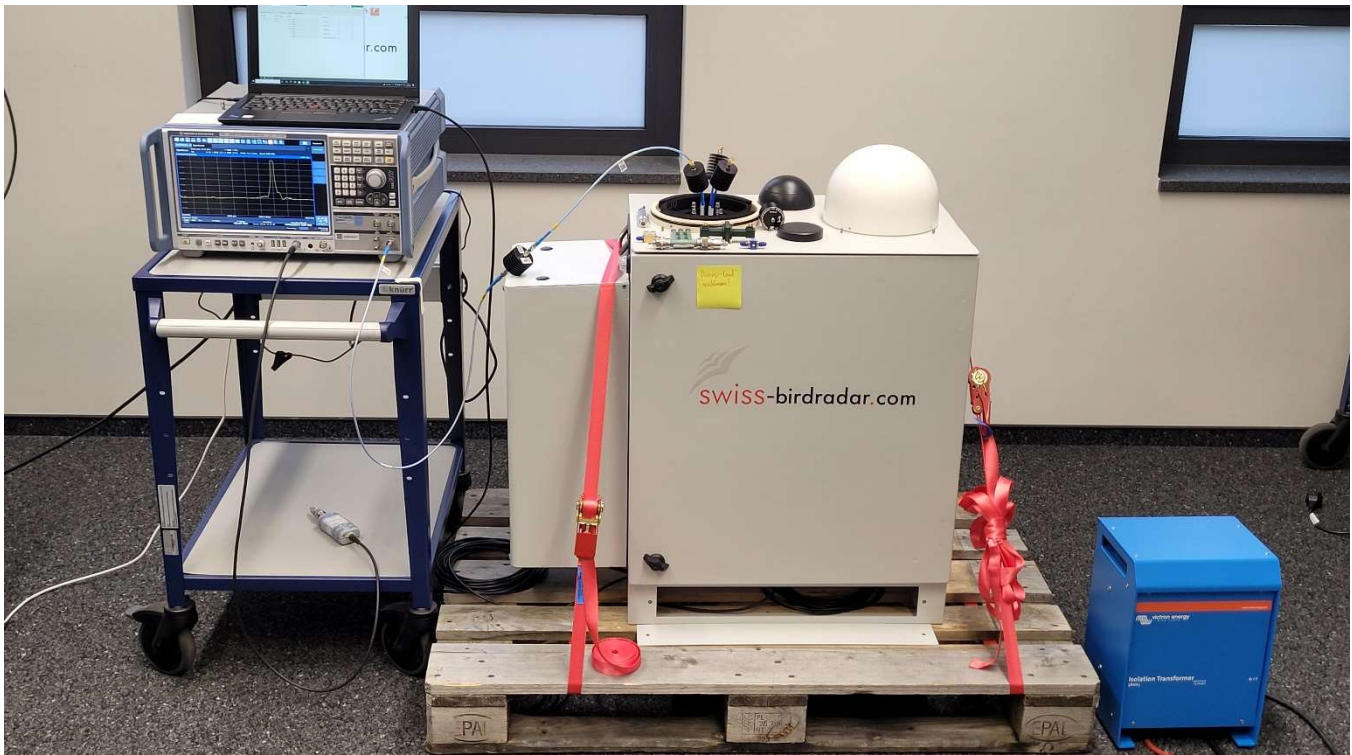
Photo No. 29: conducted RF tests
