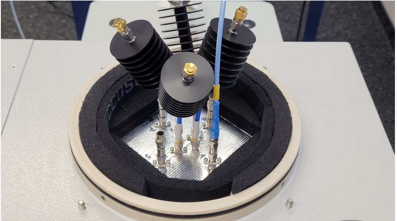
Photo No. 30: conducted RF tests
