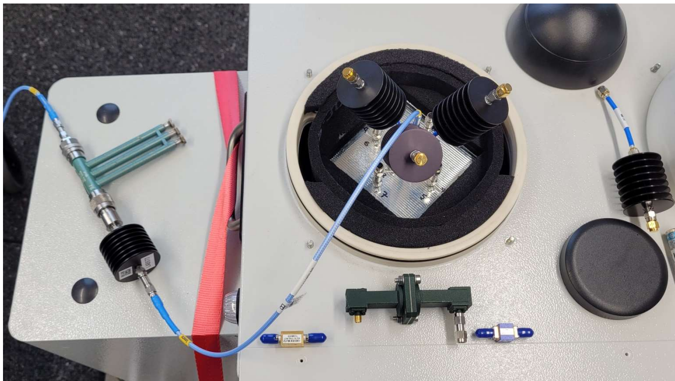
Photo No. 33: conducted RF tests with stubtuner
