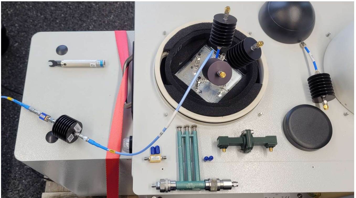
Photo No. 35: conducted RF tests with HPF
