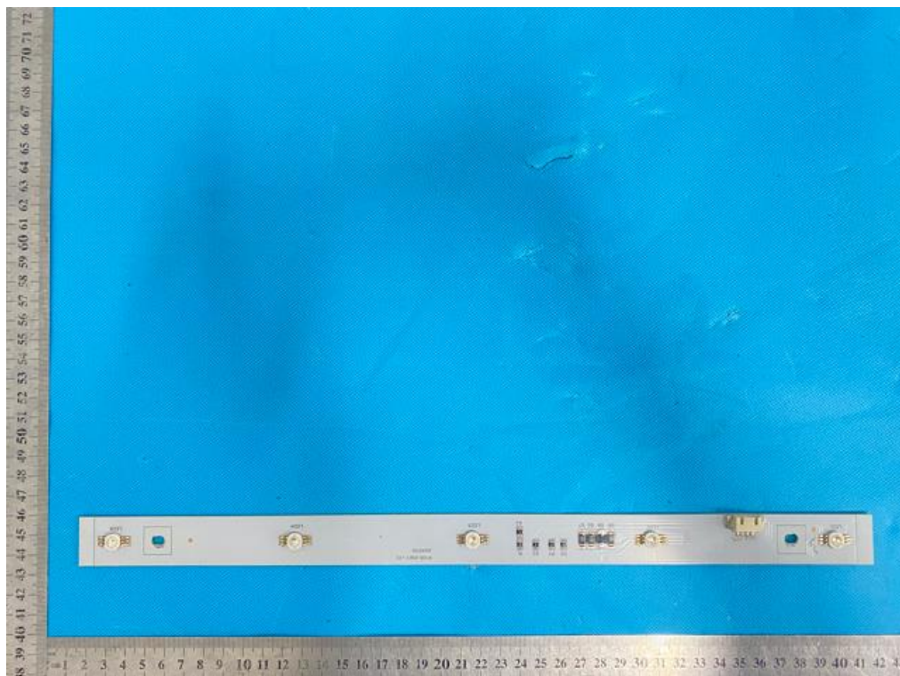
INTERNAL VIEW OF EUT (FIGURE 11) LED PCB_B
