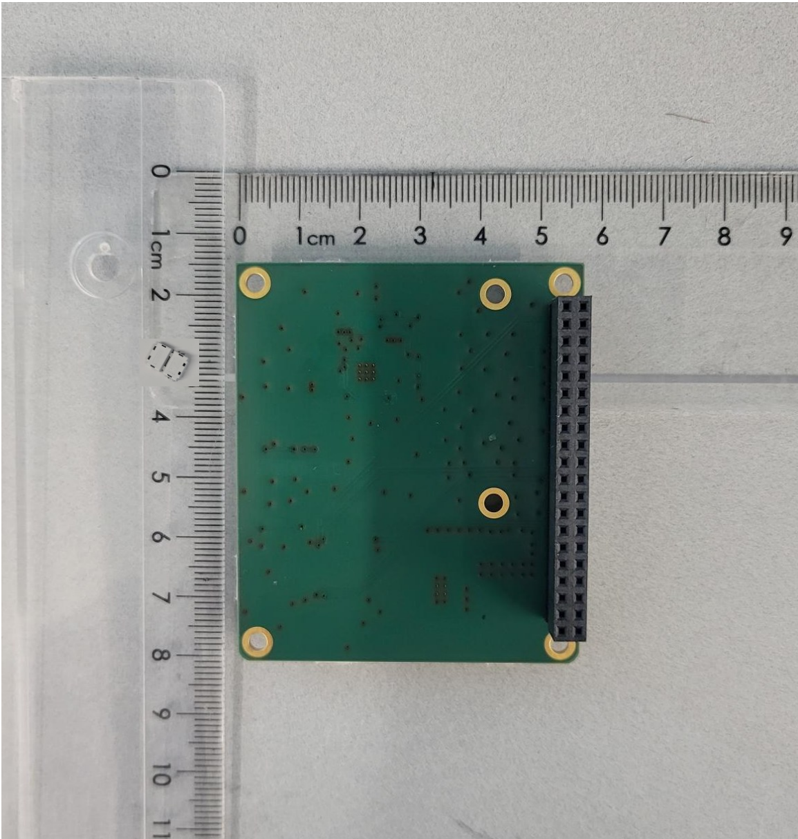
Figure 1. TSPL22-FS-PCB-V2-4 Module PCB (back)
