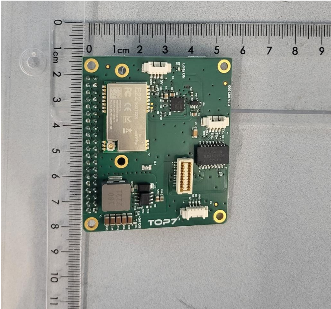
Figure 2. TSLPS22-FS-PCB-V2-4 Module PCB (front)
