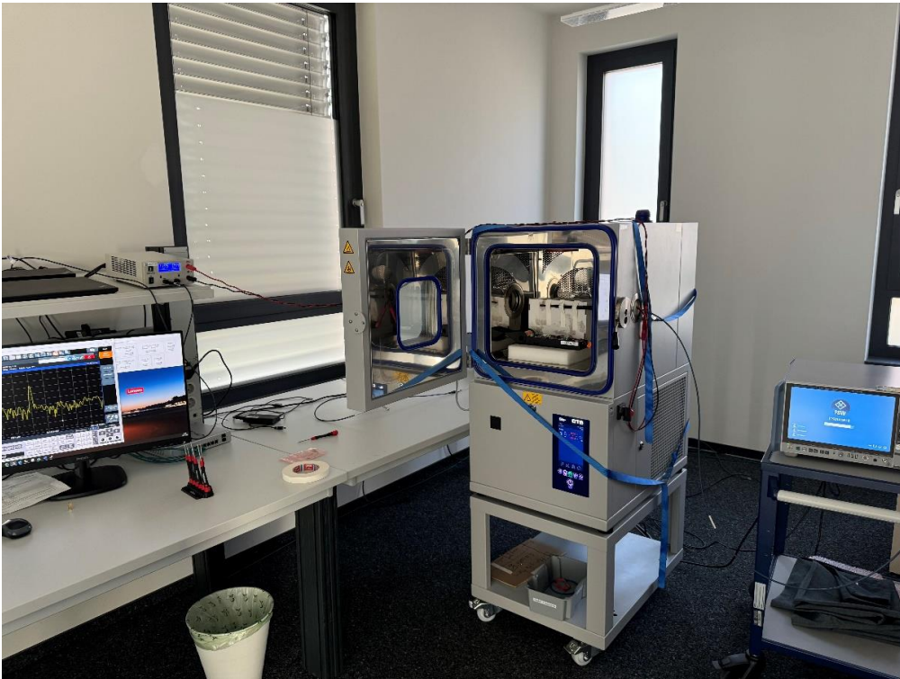
Photo No. 8, measurement in climatic chamber, overall view:
