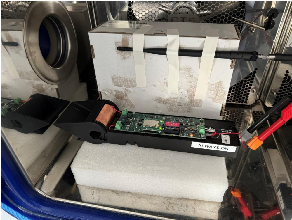
Photo No. 9, measurement in climatic chamber, close view:
