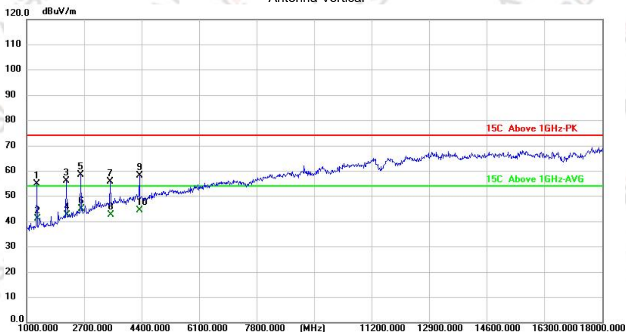
Antenna Vertical
