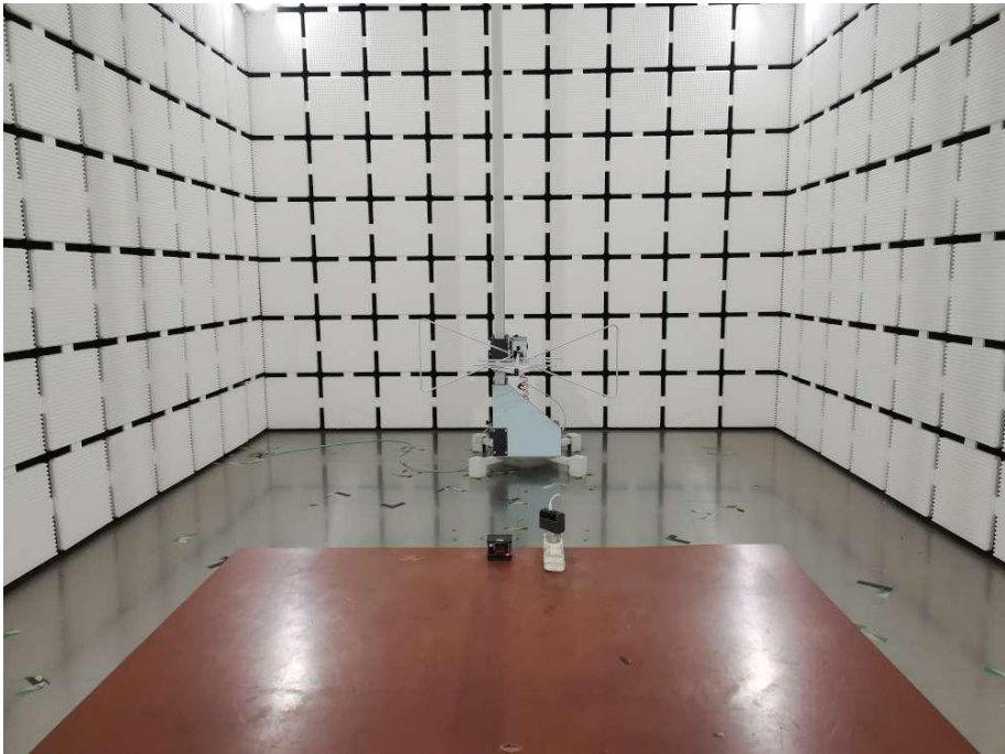
Radiated Emission Test View 2
