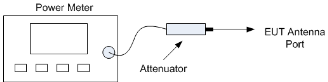
Figure 24—Example of a power meter conducted test setup
