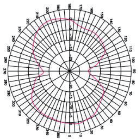
E-Plane Pattern @ 2.45GHz
