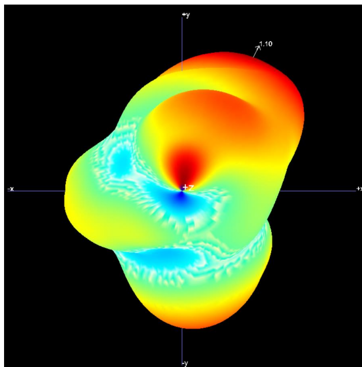
B1.3 3D Pattern for 2483.5MHz
