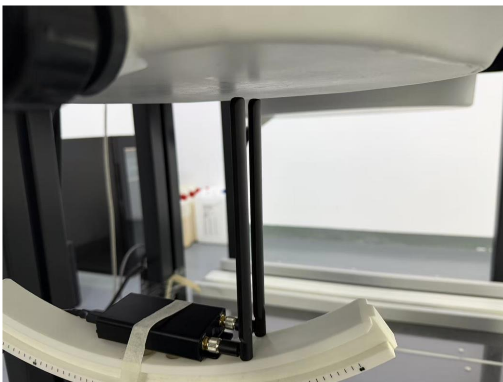
Body Right side Antenna Vertical (separation distance is 5mm)
