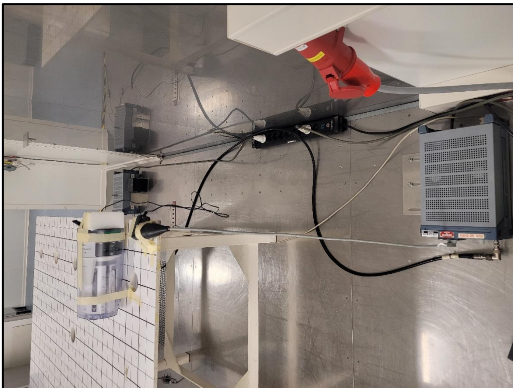
Photo 12 Conducted Test Setup
