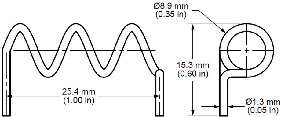
Figure 1. 916-HESM Antenna Dimensions
