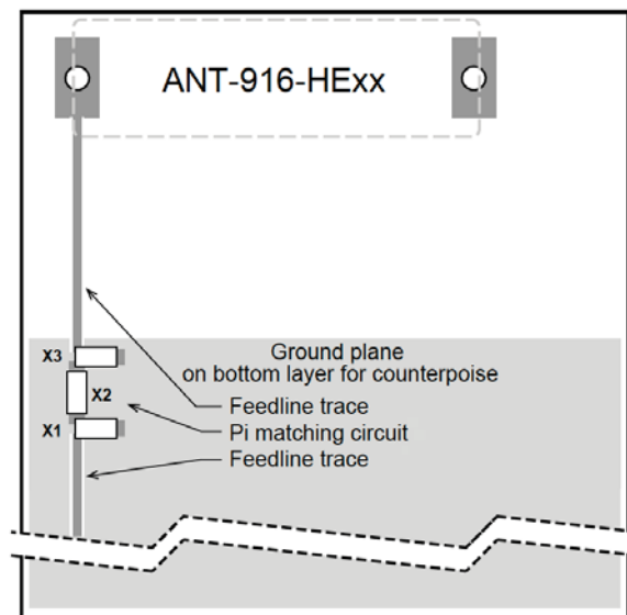
Figure 9. 916-HE Series Antenna Recommended Layout.
