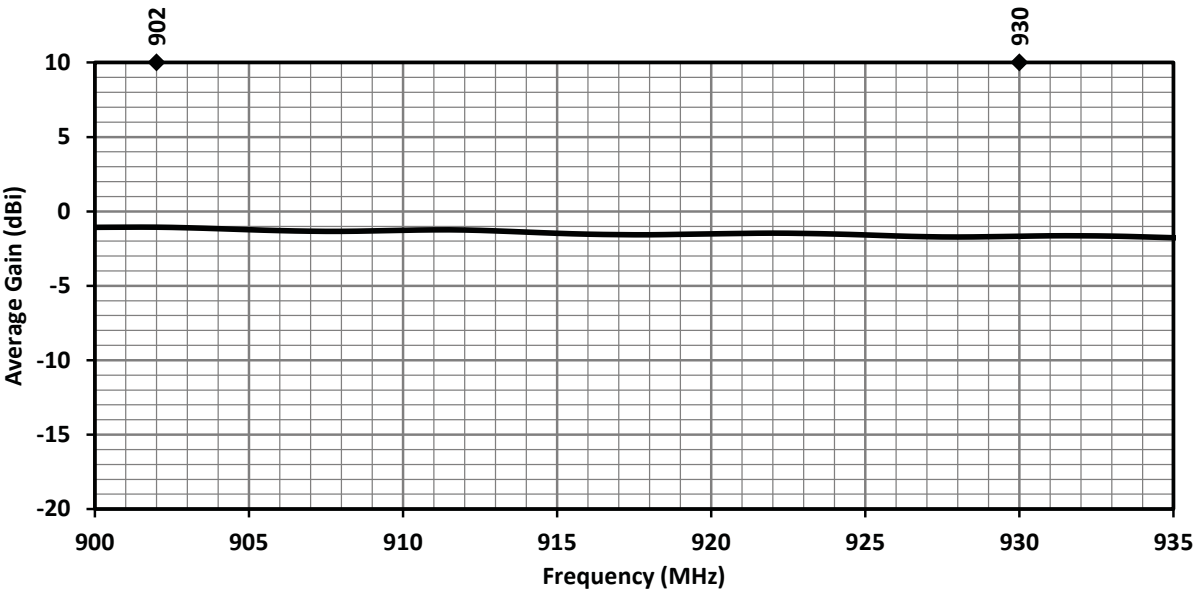
Figure 6. ANT-916-HE Series Antenna Average Gain
