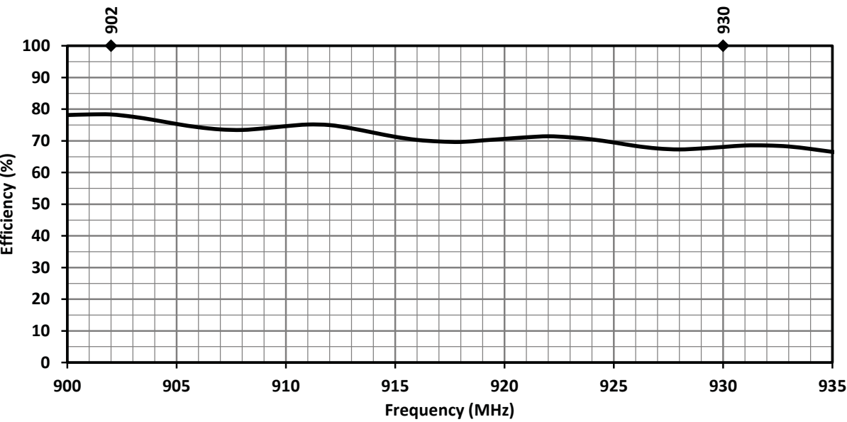
Figure 7. ANT-916-HE Series Antenna Radiation Efficiency
