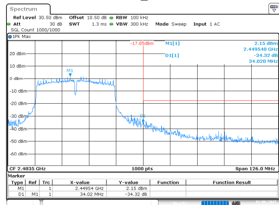
802.11n40_2452MHz
