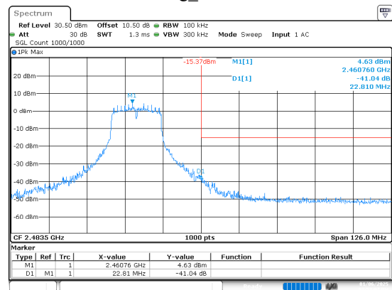
802.11g_2462MHz
