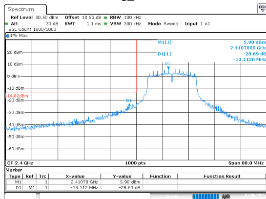
802.11g_2412MHz
