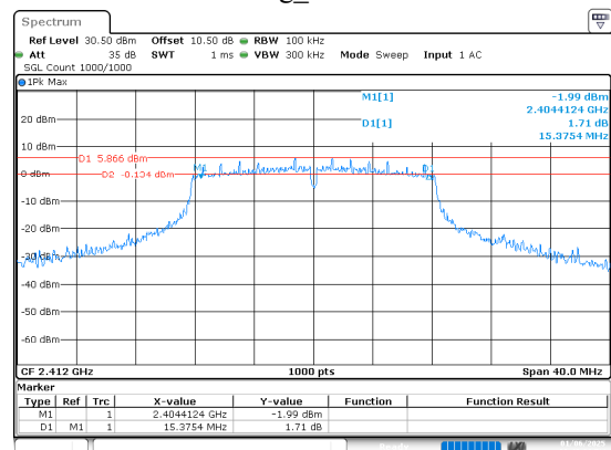
802.11g_2412MHz
