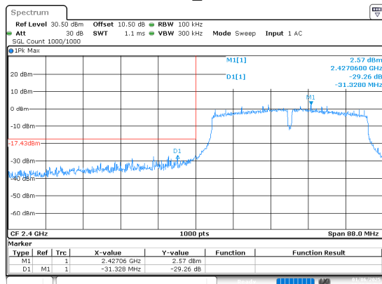
802.11n40_2422MHz
