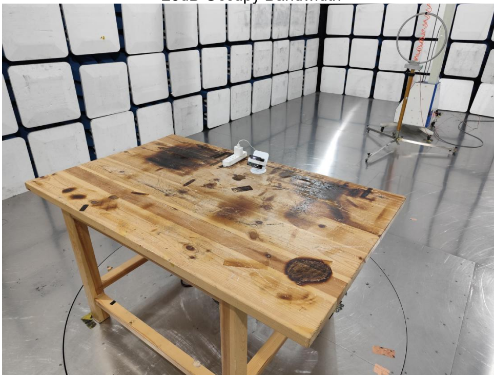
Radiation Emission Test (below 30MHz) 20dB Occupy Bandwidth
