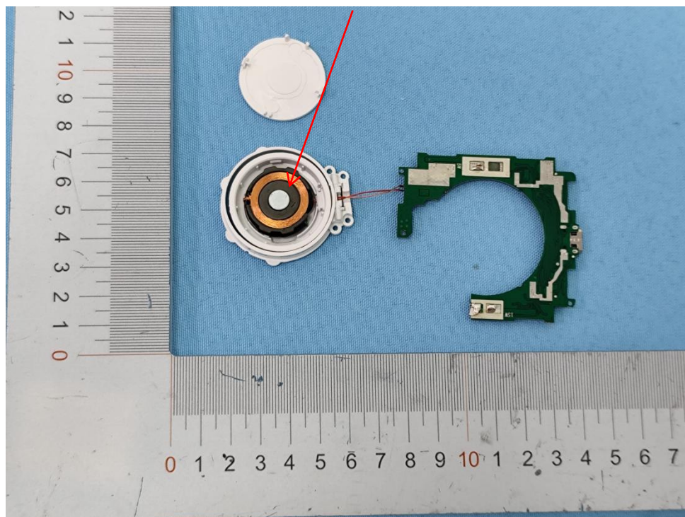
Watch-ANT
