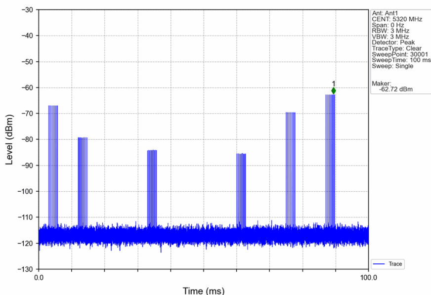
Signal Calibration_802.11ac(VHT20)_2A_5320MHz_RadarType6_Trial0
