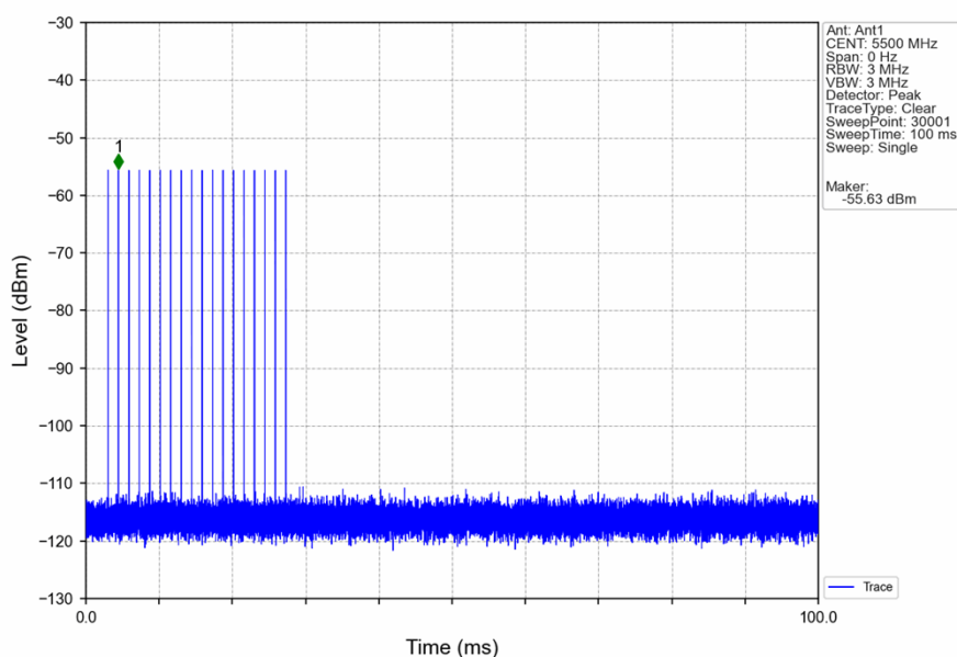
Signal Calibration_802.11ac(VHT20)_2C_5500MHz_RadarType0_Trial0
