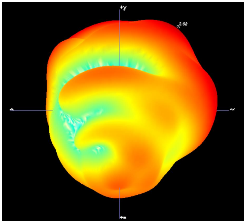
B1.2 3D Pattern for 2450MHz
