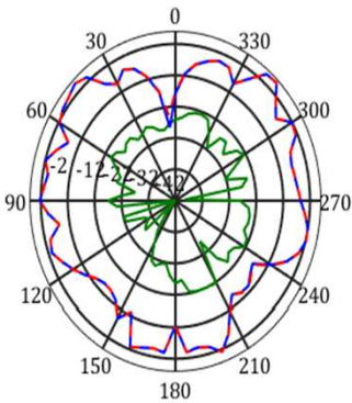
frequency=5470MHz, Y-Z Plane
