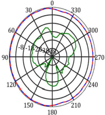
frequency=2450MHz, X-Y Plane
