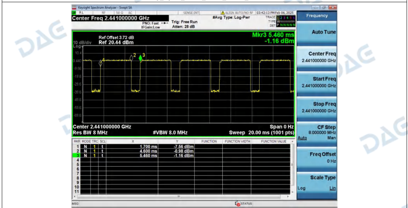
Duty_Cycle_NVNT_ANT1_3-DH5_2441
