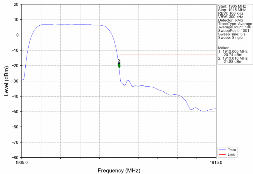
Band2_RMC_HCH_1907.6MHz_12.2kbps RMC_NTNV
