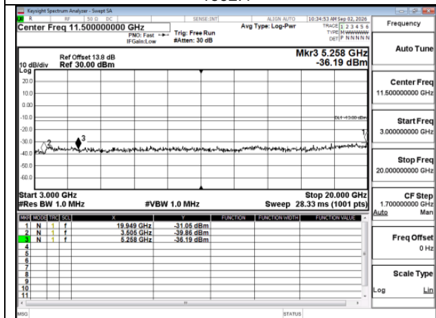
HSDPA_HSDPA_B4_High CH1513-1752.6_HighCH1513-1752.6
