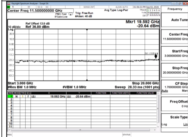
GPRS_GPRS_1900MHz_High CH810-1909.8_HighCH810-1909.8
