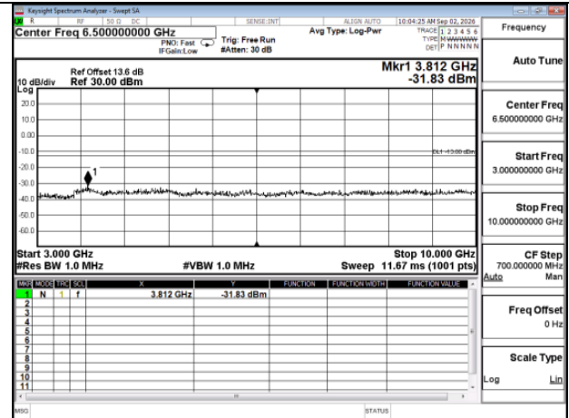
HSDPA_HSDPA_B5_Low CH4132-826.4_LowCH4132-826.4
