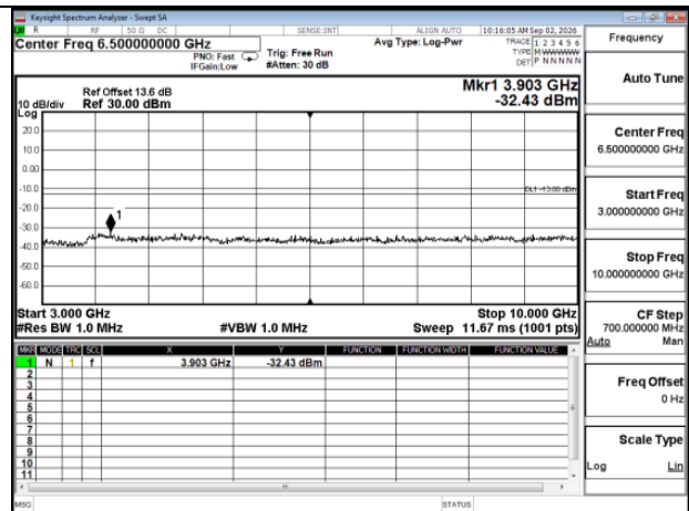
HSPA_HSPA_B5_High CH4233-846.6_HighCH4233-846.6
