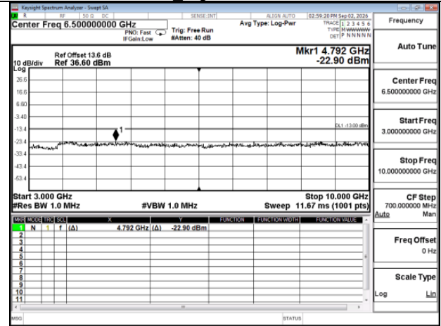
GPRS_GPRS_850MHz_Mid CH190-836.6_MidCH190-836.6
