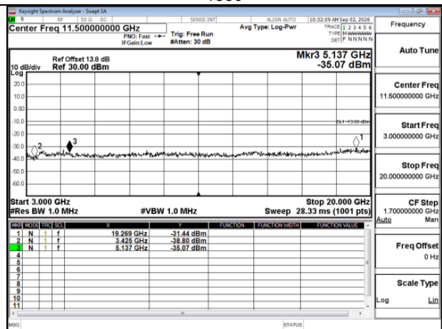
HSDPA_HSDPA_B4_Low CH1312-1712.4_LowCH1312-1712.4
