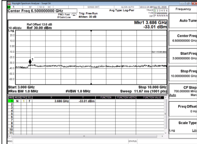
HSPA_HSPA_B5_Low CH4132-826.4_LowCH4132-826.4
