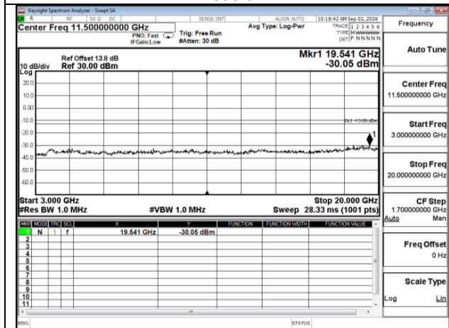
HSDPA_HSDPA_B2_Low CH9262-1852.4_LowCH9262-1852.4
