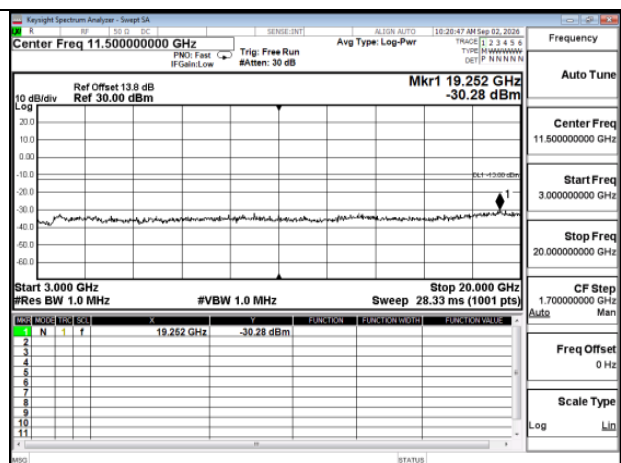
HSDPA_HSDPA_B2_High CH9538-1907.6_HighCH9538-1907.6
