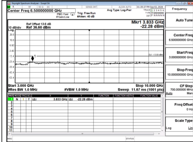
GPRS_GPRS_850MHz_Low CH128-824.2_LowCH128-824.2
