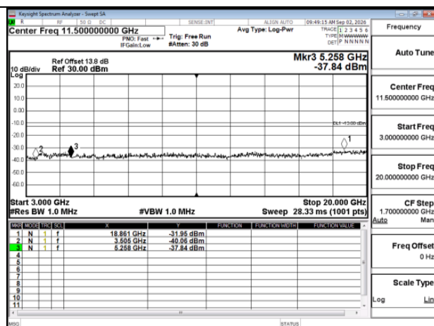
WCDMA_WCDMA_B4_High CH1513-1752.6_HighCH1513-1752.6
