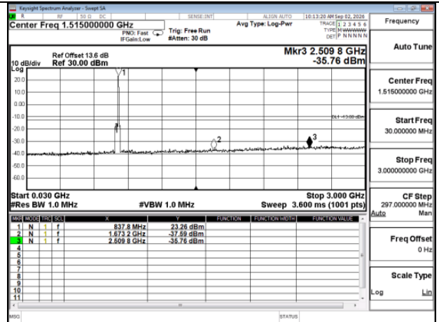
HSUPA_HSUPA_B5_Mid CH4183-836.6_MidCH4183-836.6
