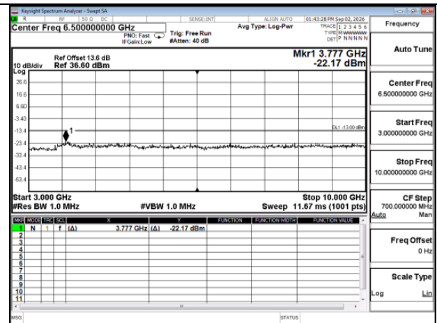
GPRS_GPRS_850MHz_High CH251-848.8_HighCH251-848.8
