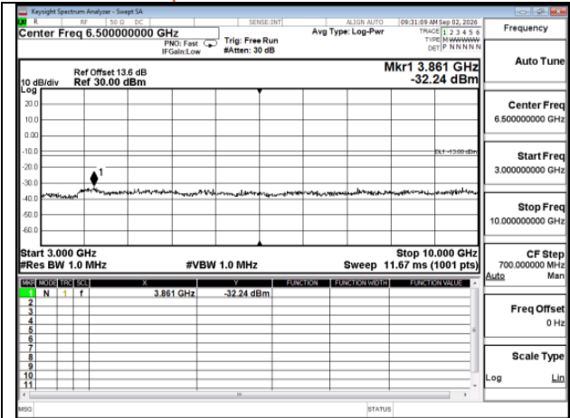
WCDMA_WCDMA_B5_Mid CH4183-836.6_MidCH4183-836.6
