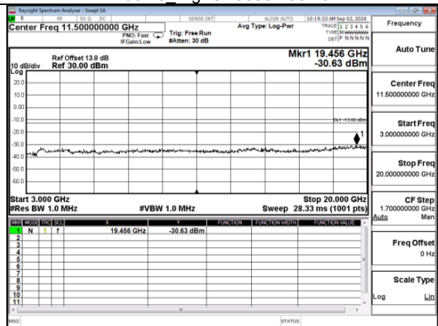
HSDPA_HSDPA_B2_Mid CH9400-1880_MidCH9400-1880
