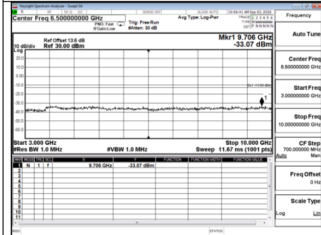
HSDPA_HSDPA_B5_High CH4233-846.6_HighCH4233-846.6
