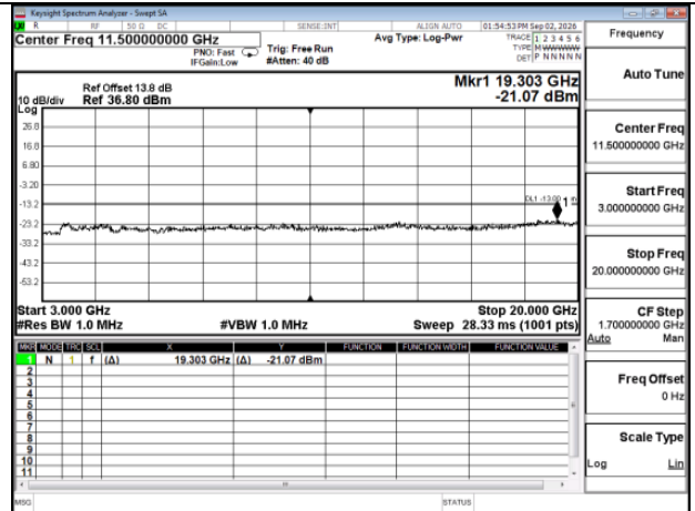
GPRS_GPRS_1900MHz_Low CH512-1850.2_LowCH512-1850.2
