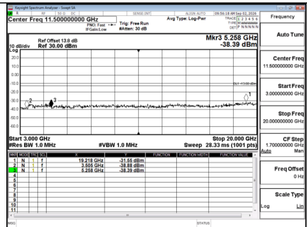
HSDPA_HSDPA_B4_High CH1513-1752.6_HighCH1513-1752.6
