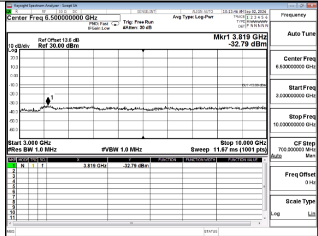
HSPA_HSPA_B5_Mid CH4183-836.6_MidCH4183-836.6
