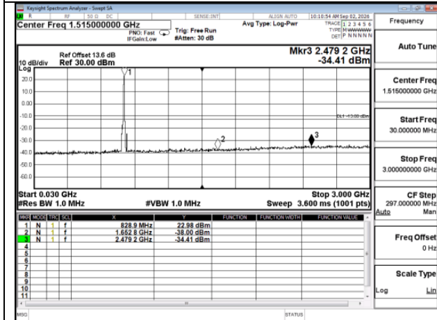
HSUPA_HSUPA_B5_Low CH4132-826.4_LowCH4132-826.4
