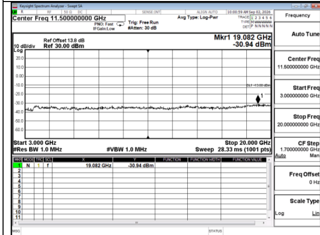
HSDPA_HSDPA_B2_High CH9538-1907.6_HighCH9538-1907.6
