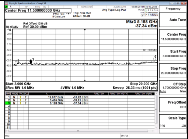
HSDPA_HSDPA_B4_Mid CH1413-1732.6_MidCH1413-1732.6
