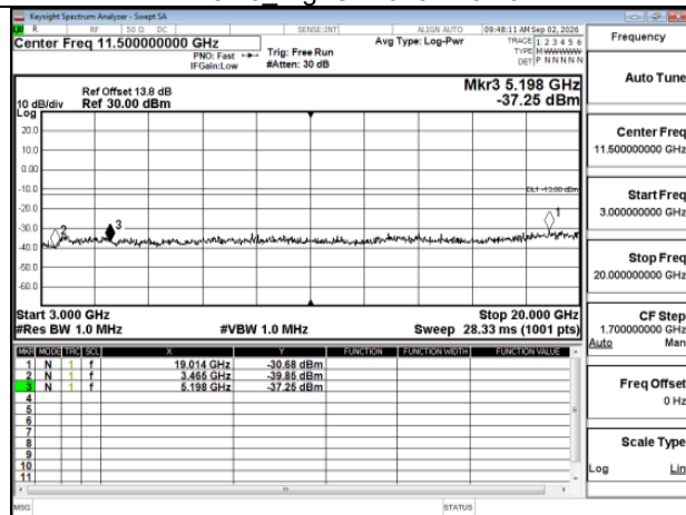
WCDMA_WCDMA_B4_Mid CH1413-1732.6_MidCH1413-1732.6
