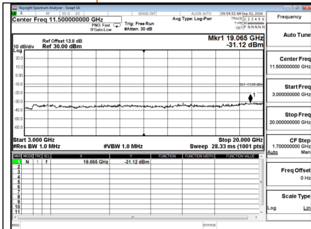
HSDPA_HSDPA_B2_Mid CH9400-1880_MidCH9400-1880
