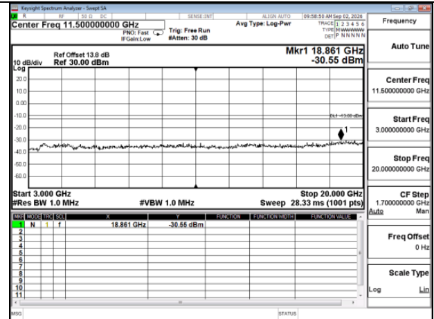
HSDPA_HSDPA_B2_Low CH9262-1852.4_LowCH9262-1852.4
