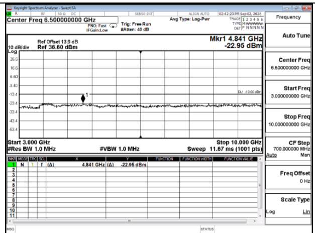
EDGE_EDGE_850MHz_High CH251-848.8_HighCH251-848.8
