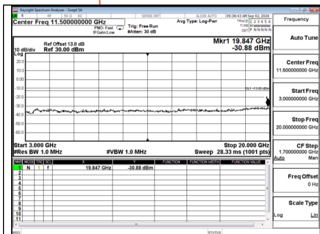
WCDMA_WCDMA_B2_Mid CH9400-1880_MidCH9400-1880
