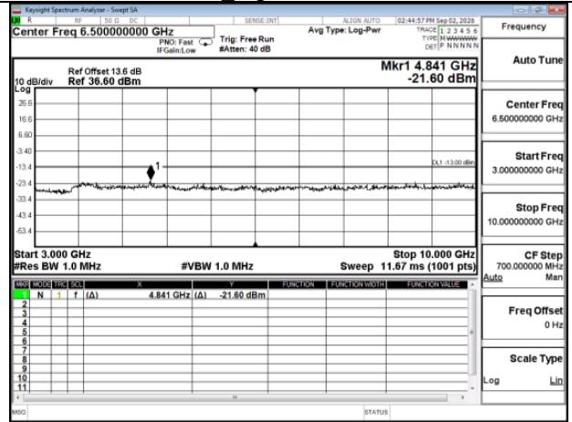
EDGE_EDGE_850MHz_Mid CH190-836.6_MidCH190-836.6
