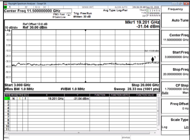
WCDMA_WCDMA_B2_Low CH9262-1852.4_LowCH9262-1852.4
