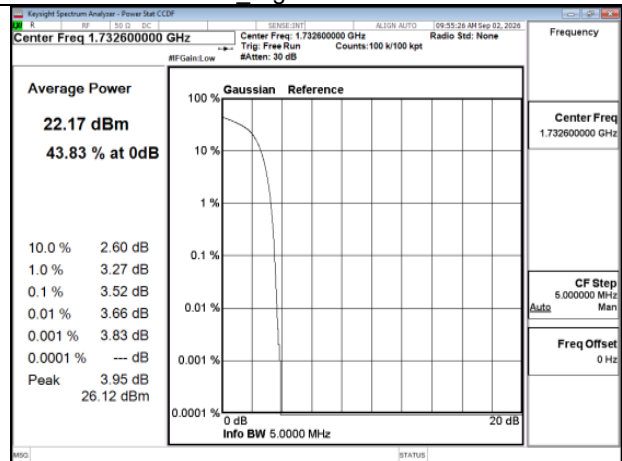
HSDPA_HSDPA_B4_Mid CH1413-1732.6_MidCH1413-1732.6
