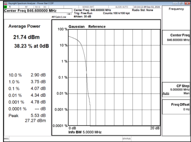
HSPA_B5_High CH4233-846.6_HighCH4233-846.6
