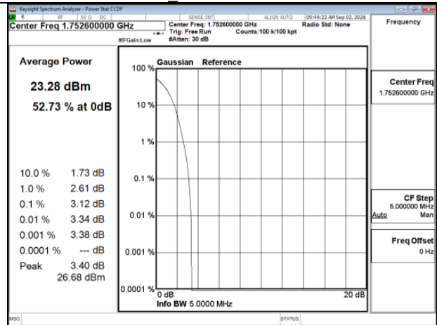
WCDMA_WCDMA_B4_High CH1513-1752.6 HighCH1513-1752.6
