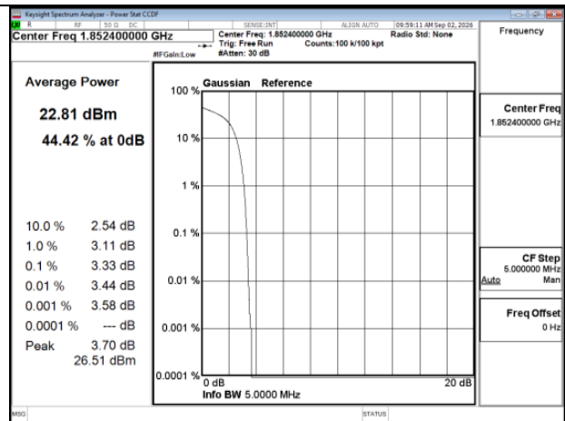
HSDPA_HSDPA_B2_Low CH9262-1852.4_LowCH9262-1852.4
