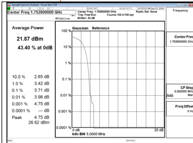
HSPA_B4_High CH1513-1752.6_HighCH1513-1752.6
