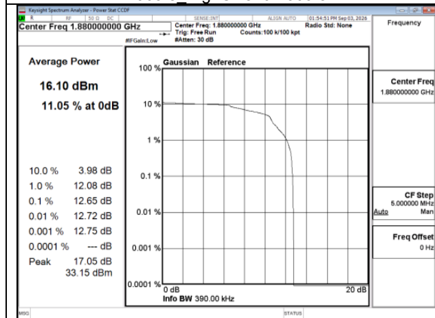
EDGE_EDGE_1900MHz_Mid CH661-1880_MidCH661-1880
