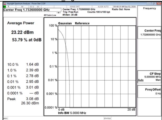
WCDMA_WCDMA_B4_Mid CH1413-1732.6 MidCH1413-1732.6
