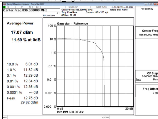
EDGE_EDGE_850MHz_Mid CH190-836.6_MidCH190-836.6
