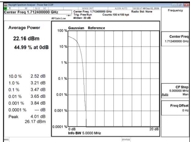
HSPA_B4_Low CH1312-1712.4_LowCH1312-1712.4
