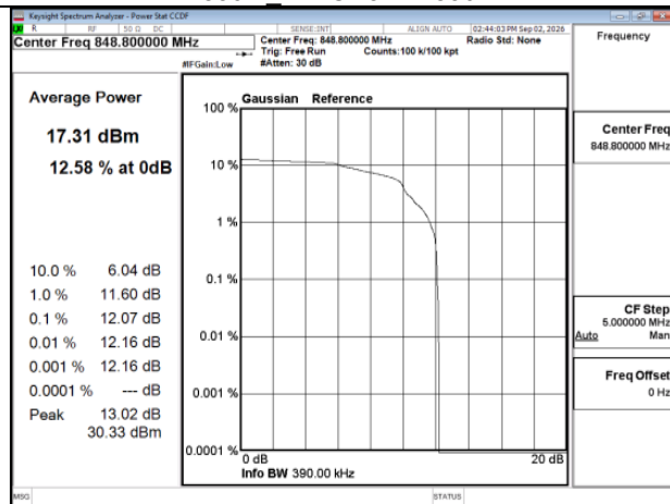
EDGE_EDGE_850MHz_High CH251-848.8 HighCH251-848.8
