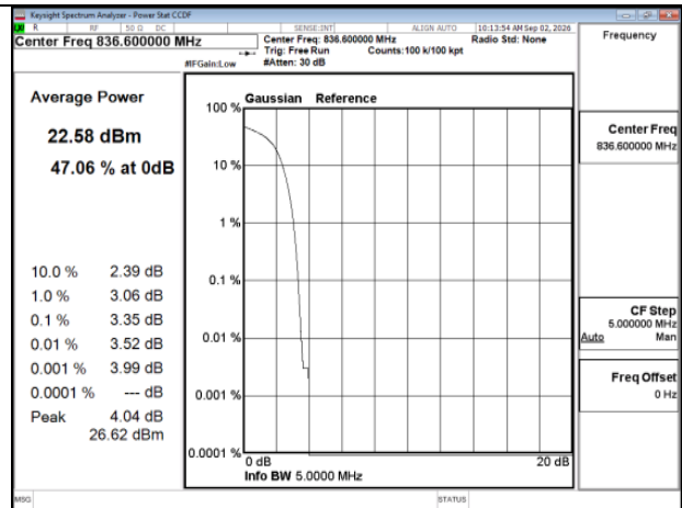
HSPA_B5_Mid CH4183-836.6_MidCH4183-836.6
