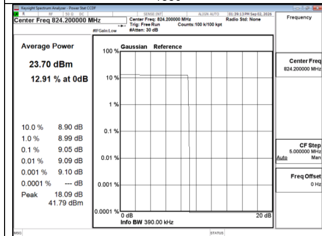
GPRS_GPRS_850MHz_Low CH128-824.2_LowCH128-824.2
