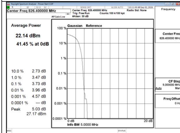
HSPA_B5_Low CH4132-826.4_LowCH4132-826.4
