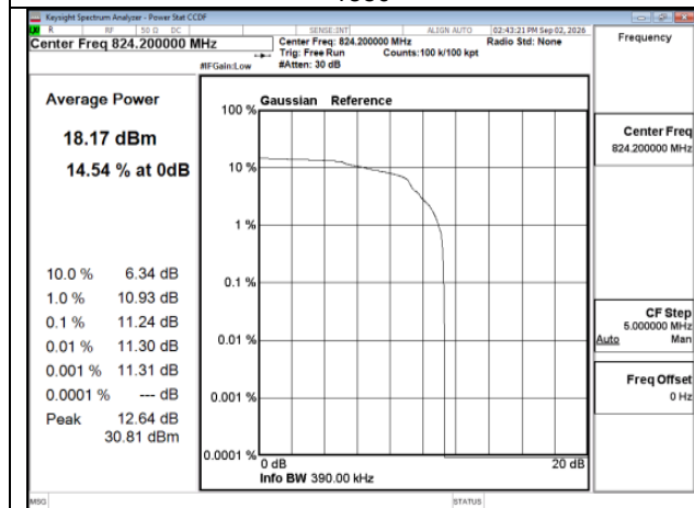
EDGE_EDGE_850MHz_Low CH128-824.2_LowCH128-824.2
