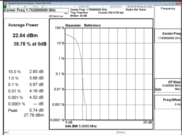
HSDPA_HSDPA_B4_High CH1513-1752.6_HighCH1513-1752.6
