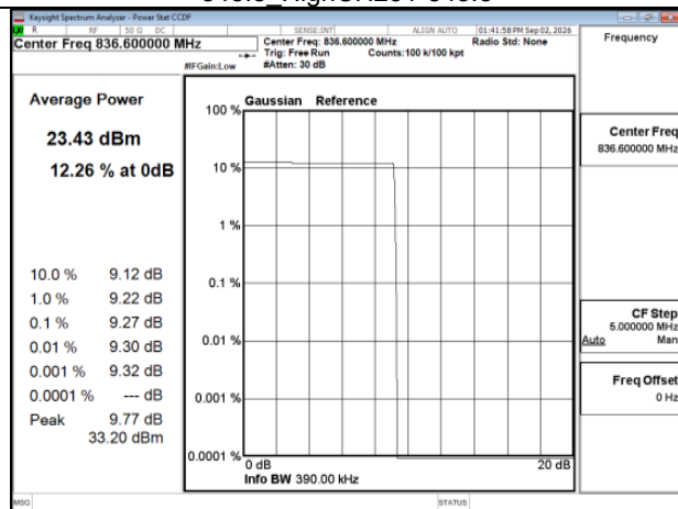
GPRS_GPRS_850MHz_Mid CH190-836.6_MidCH190-836.6
