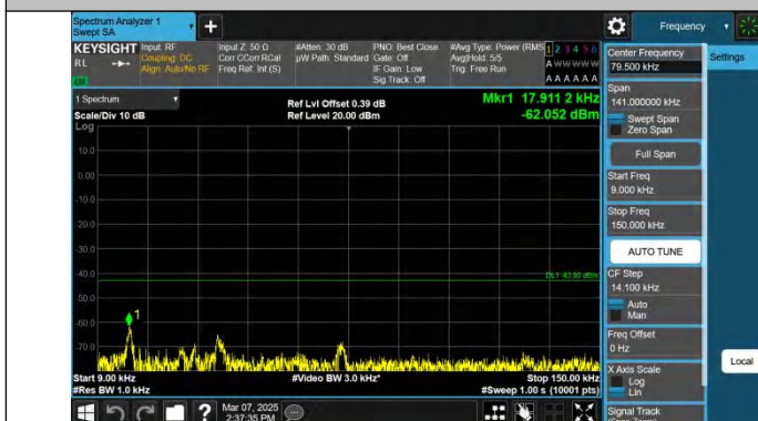
EGPRS1900-512-2-0.009~0.15MHz-PASS
