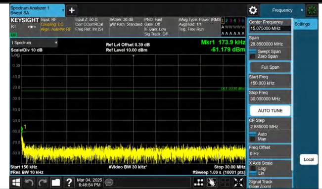
Band5-4233-5-0.15~30MHz-PASS
