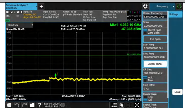
Band5-4233-5-1000~10000MHz-PASS
