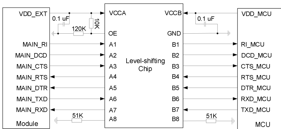
Figure 21: Reference Design of UART with a Level-shifting Chip
