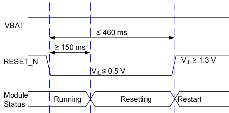
Figure 17: Reset Timing
