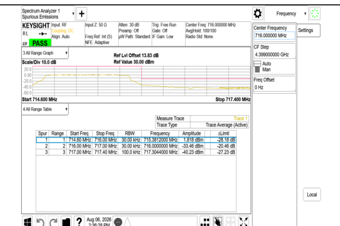
Band Edge Band12_1.4MHz_PUSCH_715.3MHz_Chain0
