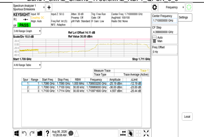
Band Edge Band4 5MHz PUSCH 1712.5MHz Chain0
