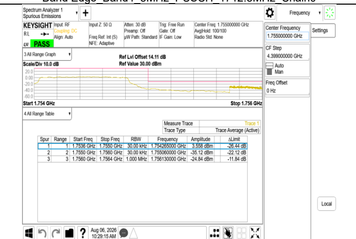
Band Edge Band4 5MHz PUSCH 1752.5MHz Chain0
