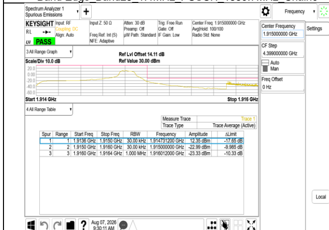
Band Edge Band25 1.4MHz PUSCH 1914.3MHz Chain0
