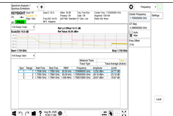
Band Edge Band4 15MHz PUSCH 1747.5MHz Chain0
