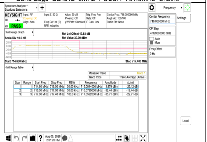
Band Edge Band12 5MHz PUSCH 713.5MHz Chain0
