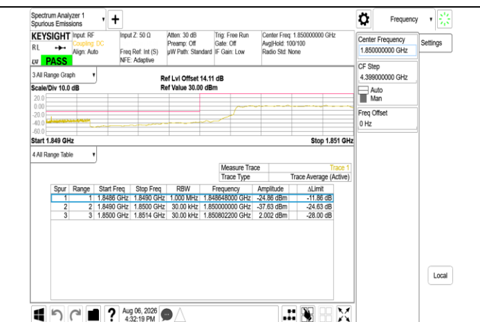
Band25 3MHz Chain0 1851.5MHz NBI 0 QPSK 6 0
