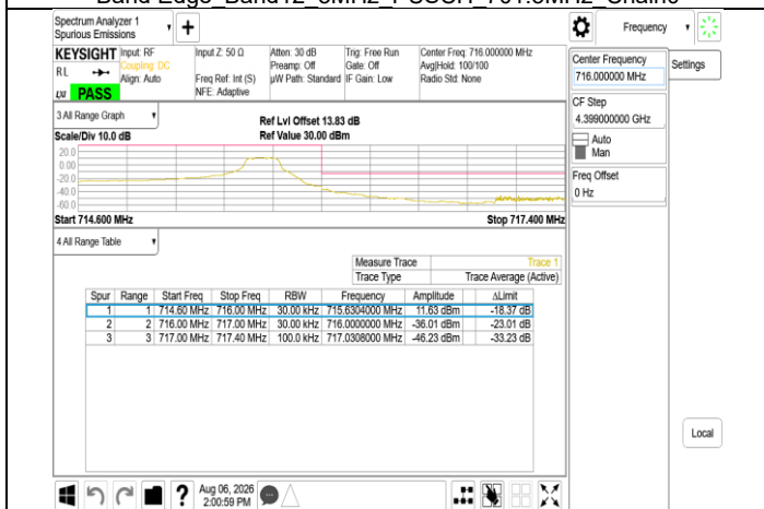
Band Edge Band12 5MHz PUSCH 713.5MHz Chain0
