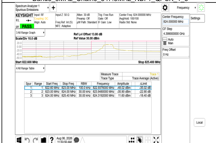
Band Edge Band5 5MHz PUSCH 826.5MHz Chain0
