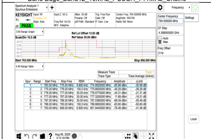
Band Edge Band13 5MHz PUSCH 779.5MHz Chain0
