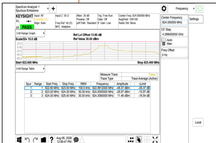
Band Edge Band5 1.4MHz PUSCH 824.7MHz Chain0
