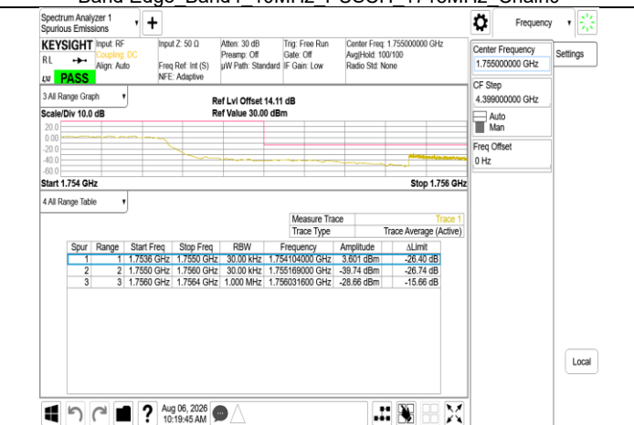
Band Edge Band4 10MHz PUSCH 1750MHz Chain0
