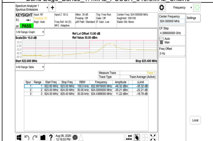
Band5 3MHz Chain0 825.5MHz NBI 0 QPSK 1 0
