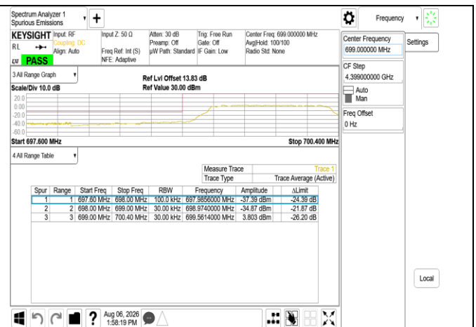
Band Edge Band12 5MHz PUSCH 701.5MHz Chain0
