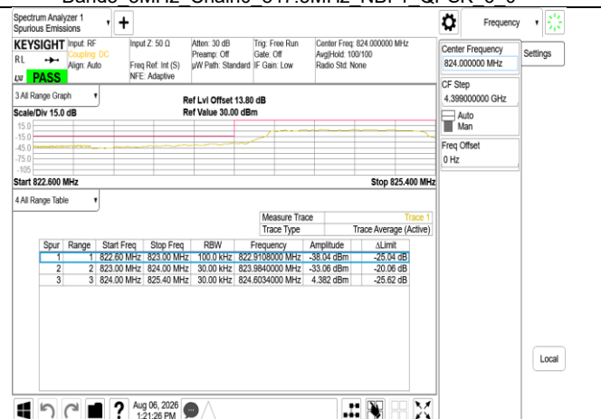
Band Edge Band5 5MHz PUSCH 826.5MHz Chain0
