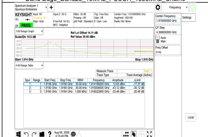
Band Edge Band25_10MHz_PUSCH_1910MHz_Chain0
