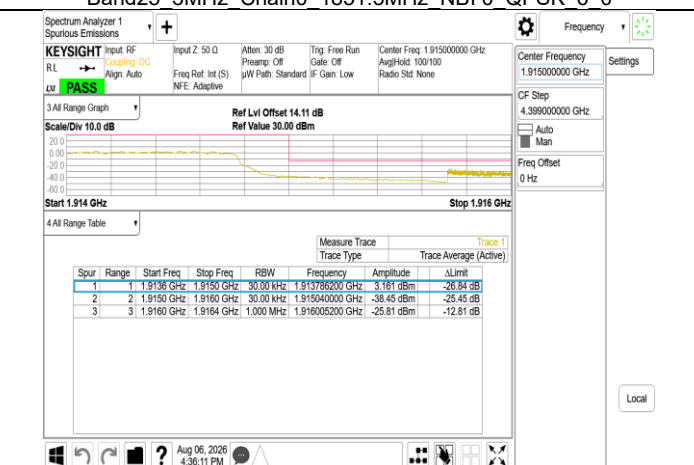
Band25 3MHz Chain0 1913.5MHz NBI 1 QPSK 6 0
