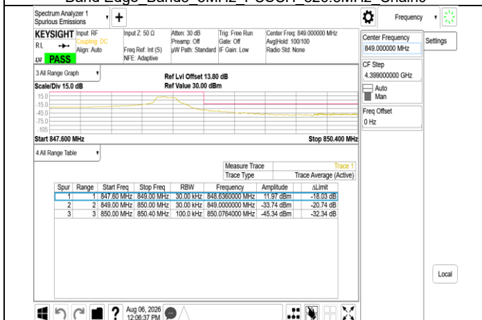
Band Edge Band5 5MHz PUSCH 846.5MHz Chain0
