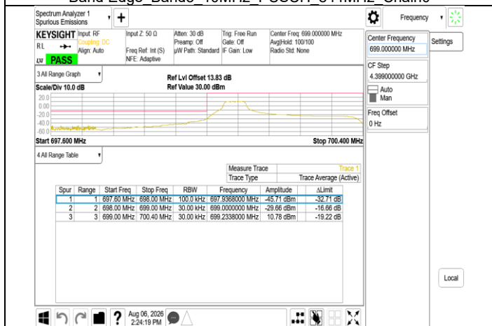
Band Edge Band12 1.4MHz PUSCH 699.7MHz Chain0
