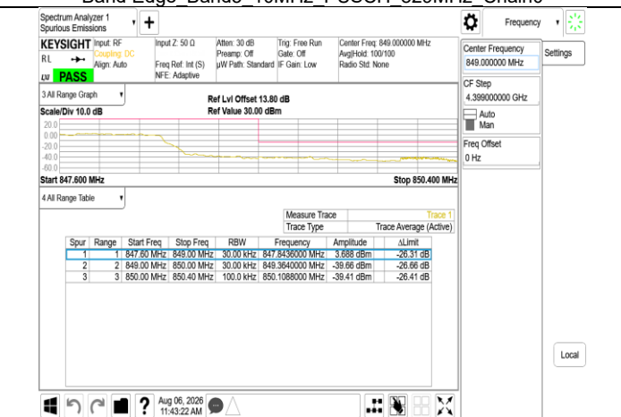
Band Edge Band5 10MHz PUSCH 844MHz Chain0
