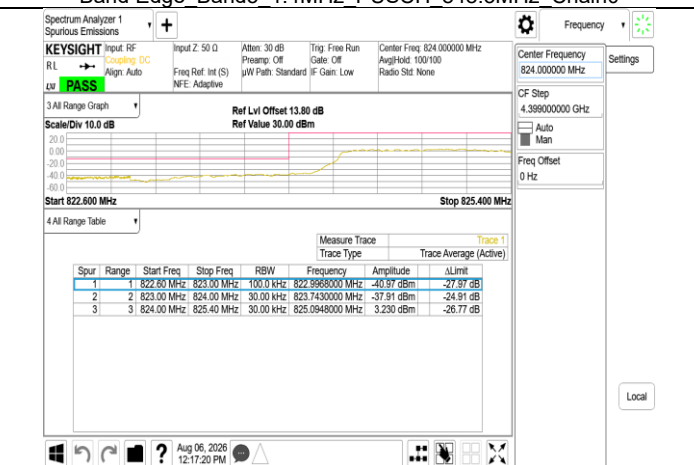
Band5 3MHz Chain0 825.5MHz NBI 0 QPSK 6 0
