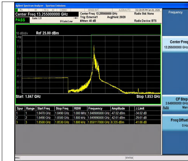
Band25-0.18-BPSK-26042-PASS
