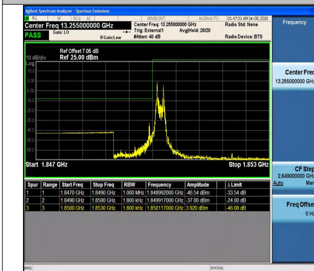
Band25-0.18-BPSK-26042-PASS
