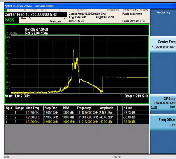
Band25-0.18-QPSK-26688-PASS
