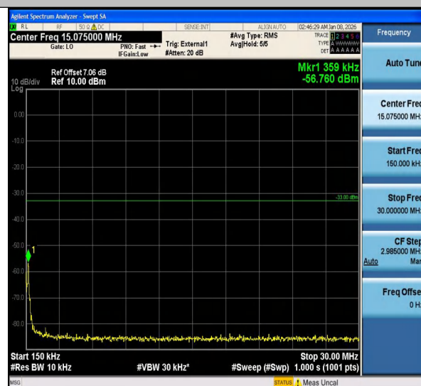
Band25-0.18-BPSK-26688-0.15-30-PASS
