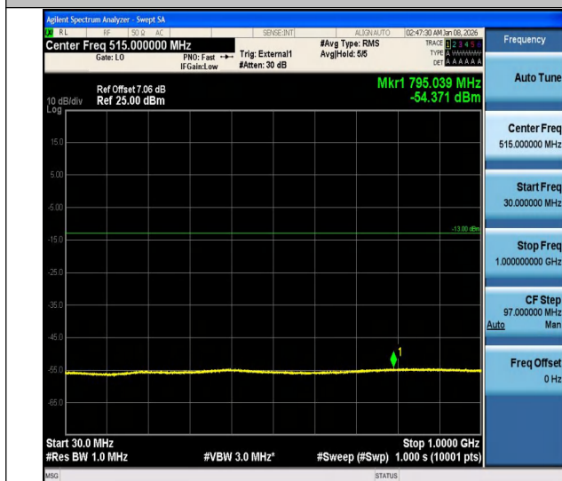
Band25-0.18-BPSK-26688-30-1000-PASS
