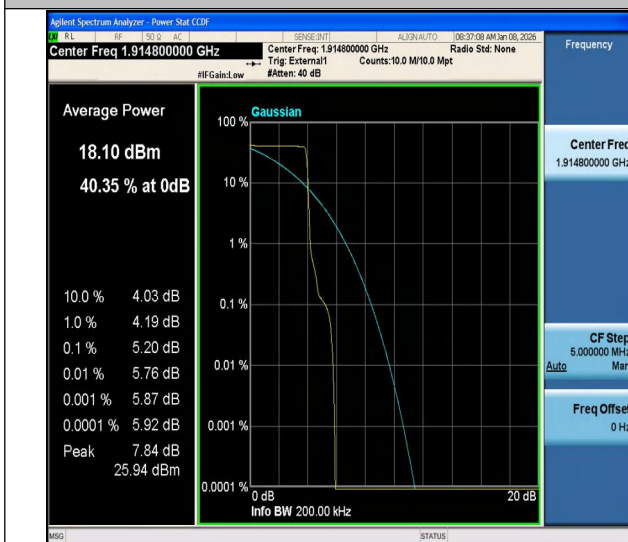
Band25-0.18-QPSK-26688-PASS
