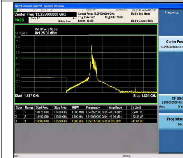
Band25-0.18-QPSK-26042-PASS
