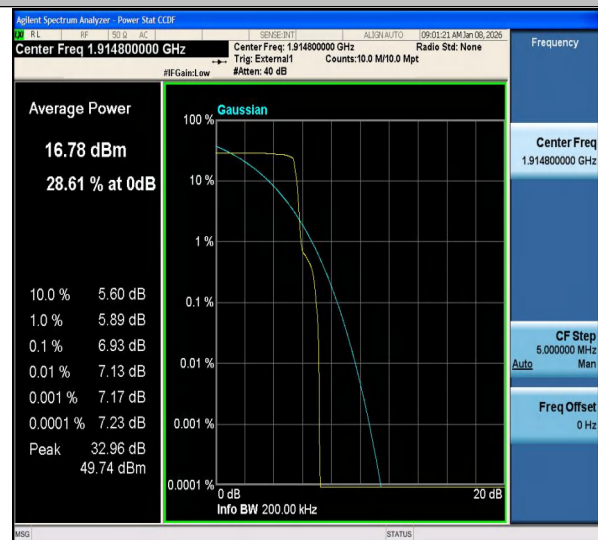
Band25-0.18-QPSK-26688-PASS
