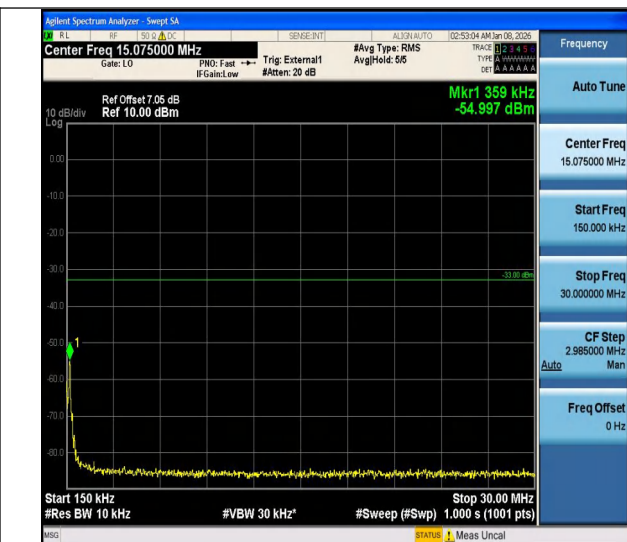
Band25-0.18-BPSK-26042-0.15-30-PASS
