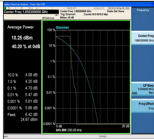
Band25-0.18-QPSK-26042-PASS
