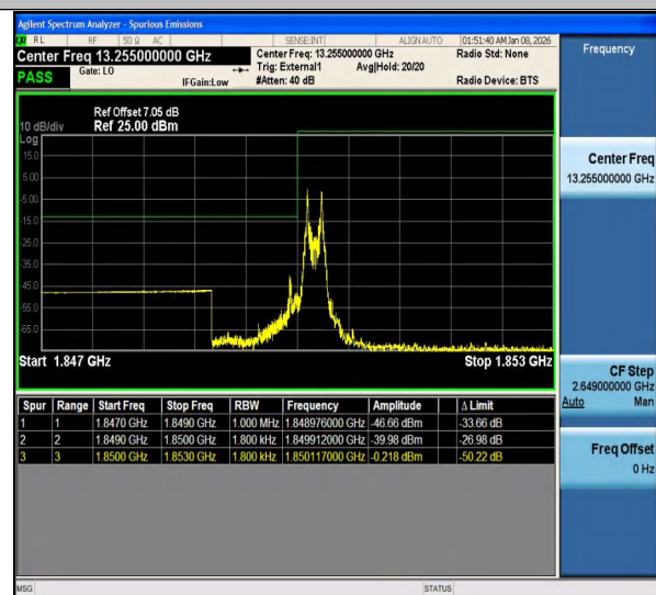
Band25-0.18-QPSK-26042-PASS
