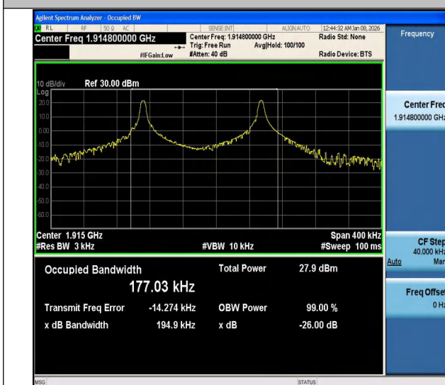
Band25-0.18-BPSK-26688-PASS
