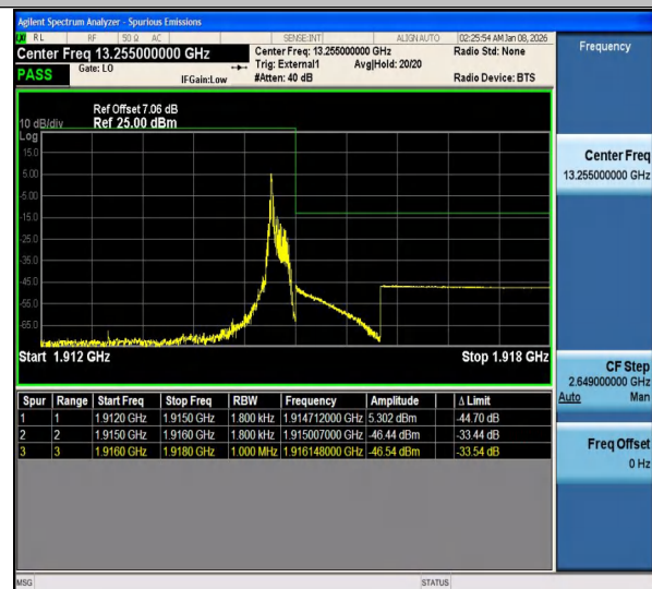
Band25-0.18-BPSK-26688-PASS
