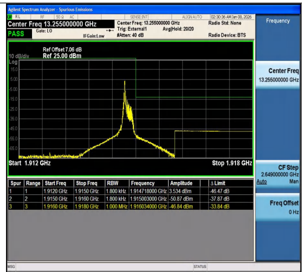
Band25-0.18-QPSK-26688-PASS
