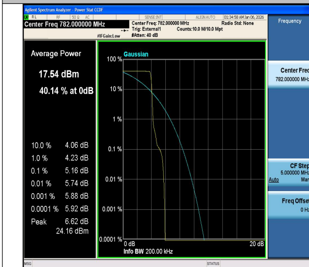
Band13-0.18-QPSK-23230-PASS
