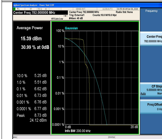
Band13-0.18-QPSK-23230-PASS
