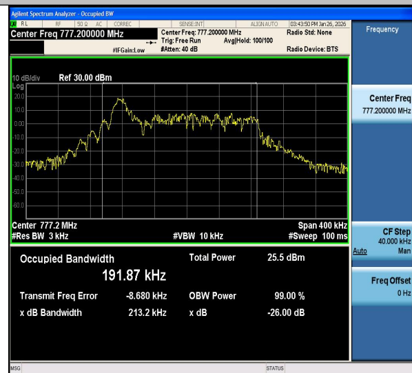
Band13-0.18-QPSK-23182-PASS
