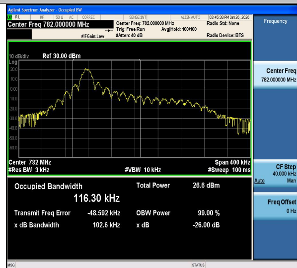
Band13-0.18-QPSK-23230-PASS
