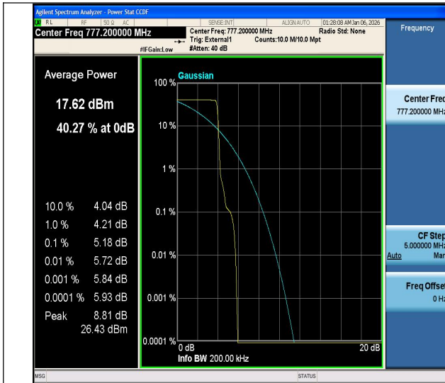
Band13-0.18-QPSK-23182-PASS
