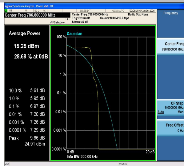
Band13-0.18-QPSK-23278-PASS
