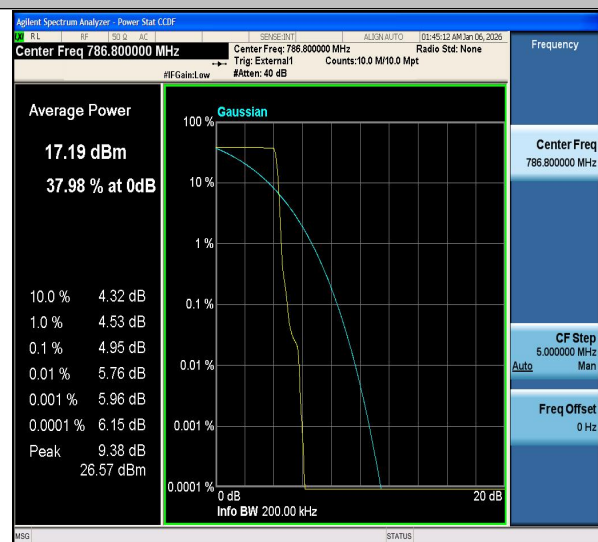
Band13-0.18-QPSK-23278-PASS
