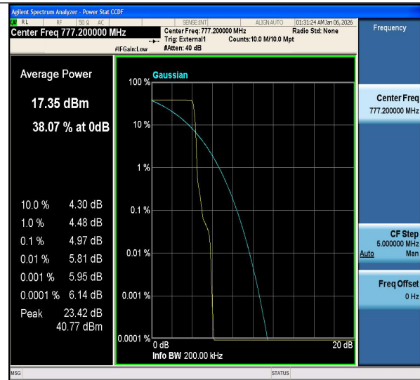
Band13-0.18-QPSK-23182-PASS
