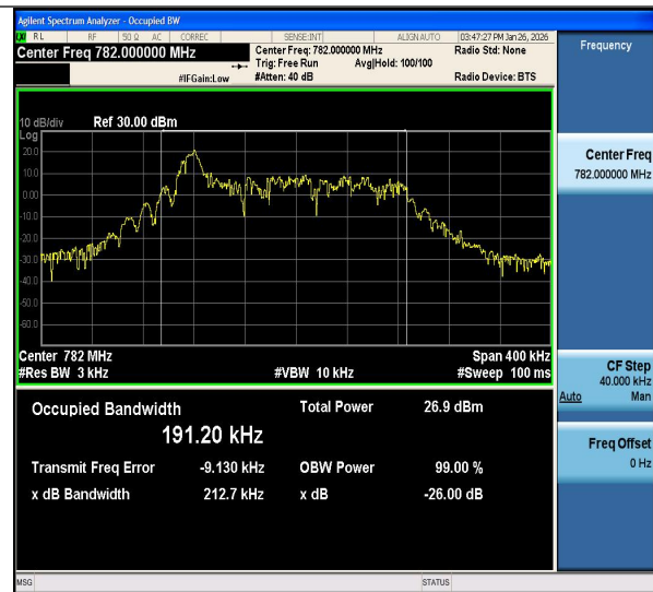
Band13-0.18-QPSK-23230-PASS
