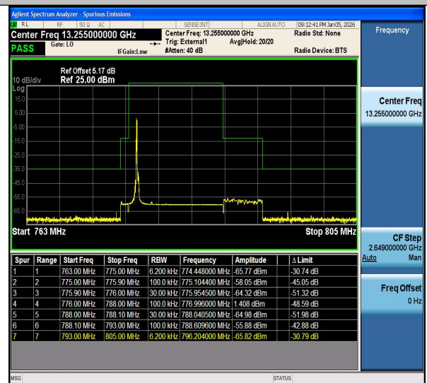
Band13-0.18-QPSK-23181-PASS
