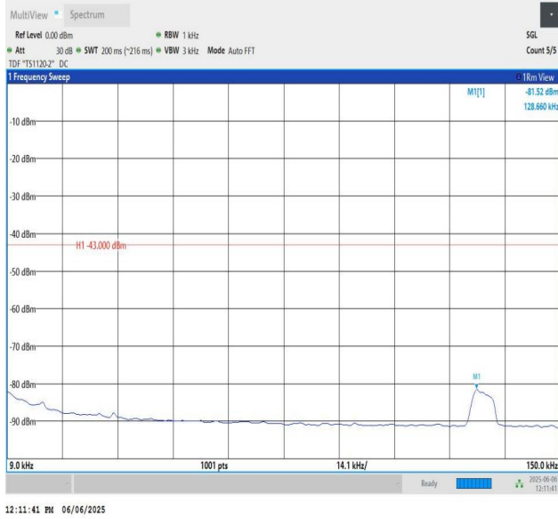
Band4-20MHz-QPSK-20175-PASS
