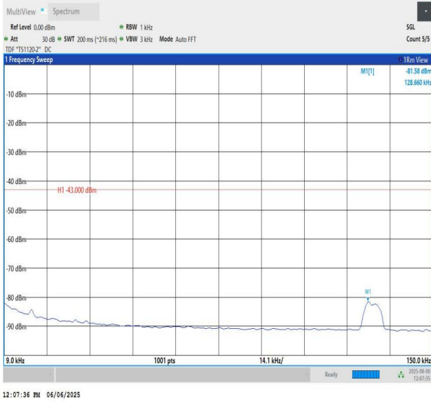
Band4-15MHz-QPSK-20175-PASS
