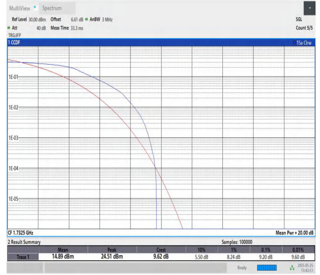
Band4-3MHz-16QAM-20175-PASS
