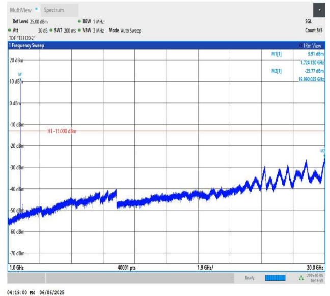
Band4-20MHz-QPSK-20175-PASS
