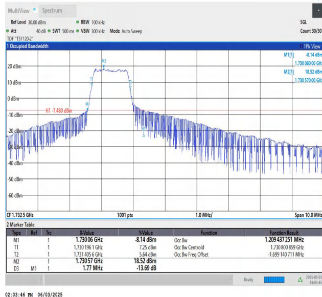
Band4-5MHz-16QAM-20175-PASS
