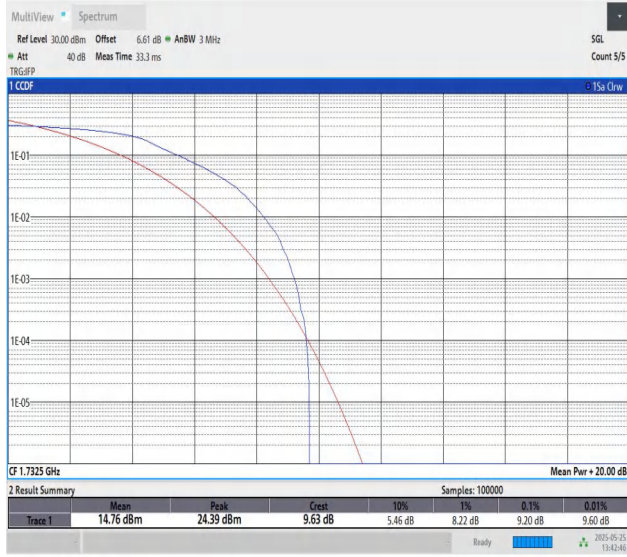
Band4-3MHz-QPSK-20175-PASS
